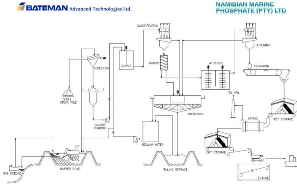
Figure 13 - Simplified concentrate production flow sheet
