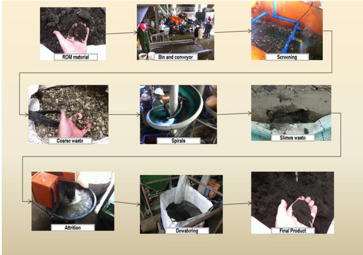
Figure 12 - Beneficiation process
