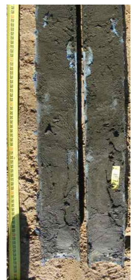
Figure 9 - Typical sedimentary sequence of the deposits with core 1877 showing both layers 1 and 2 of the deposit.
