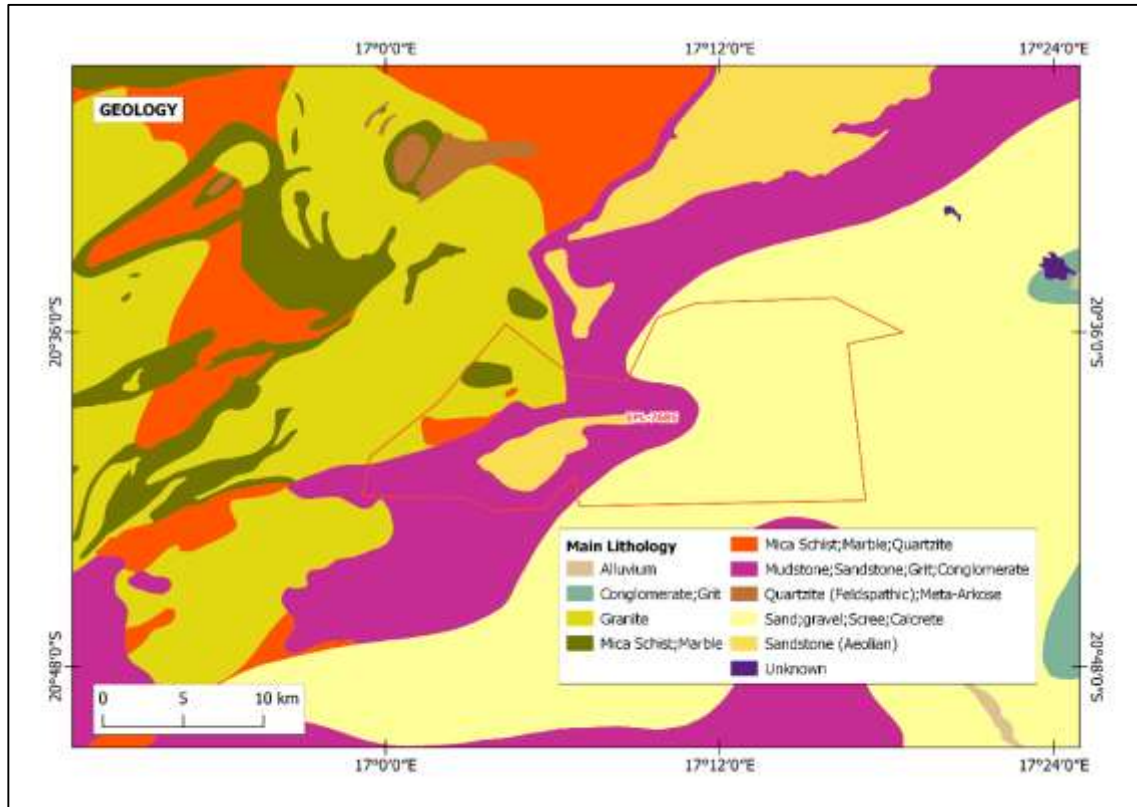
Figure 4: The geology of the EPL
