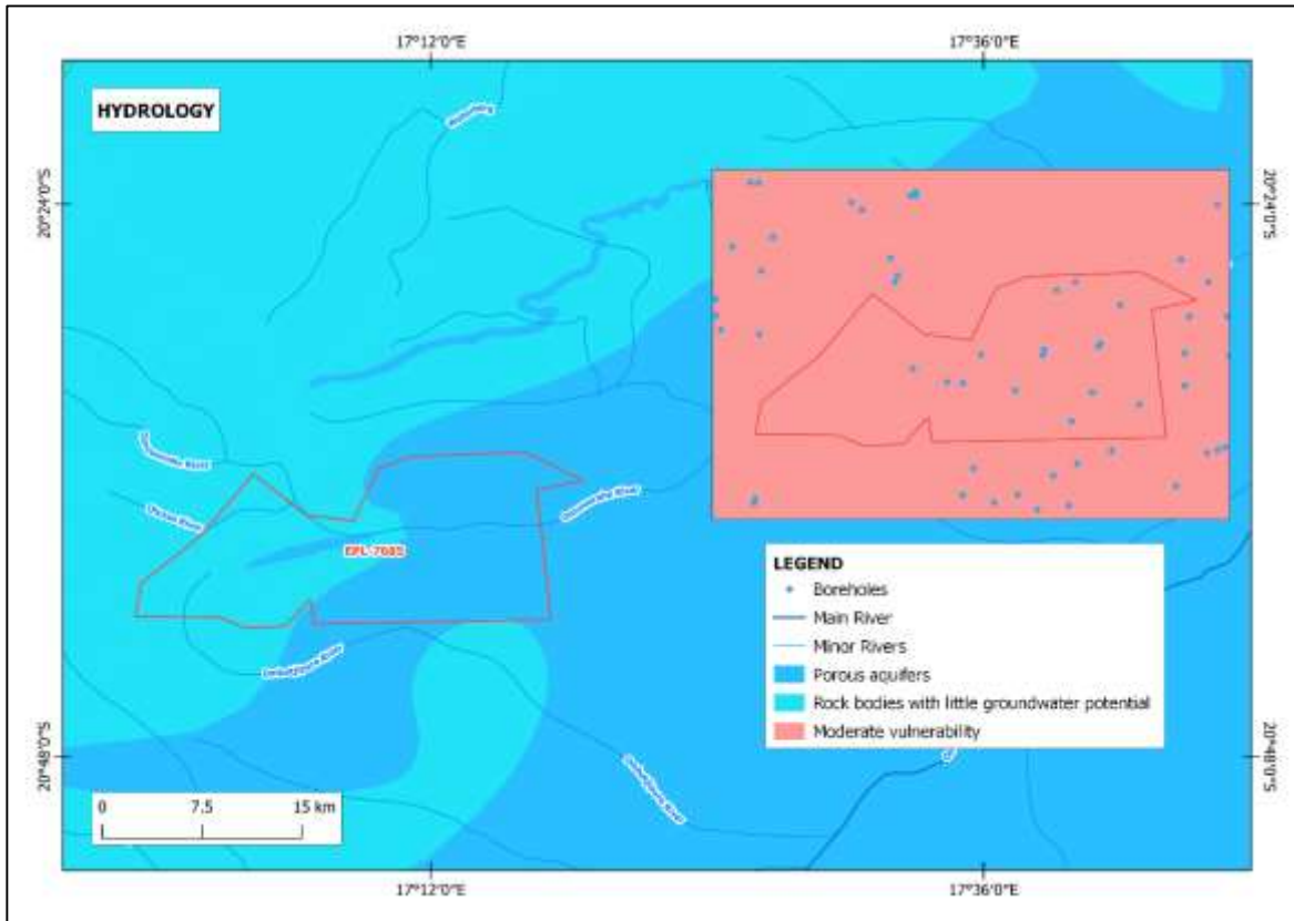
Figure 6: Shows the groundwater map for the EPL
