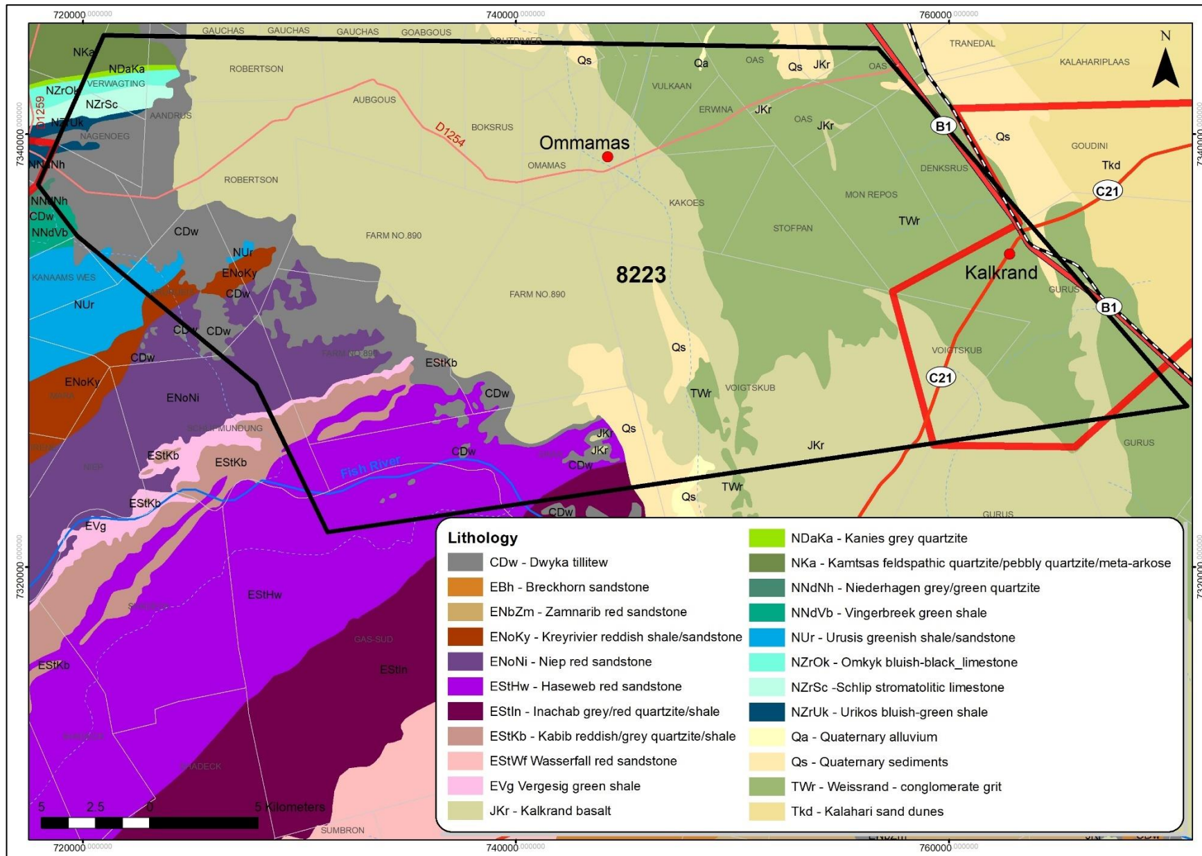
Figure 6: Simplified local geological map of the EPL 8223 (RBS Map Prepared by Katharina Dierkes, 2021).
