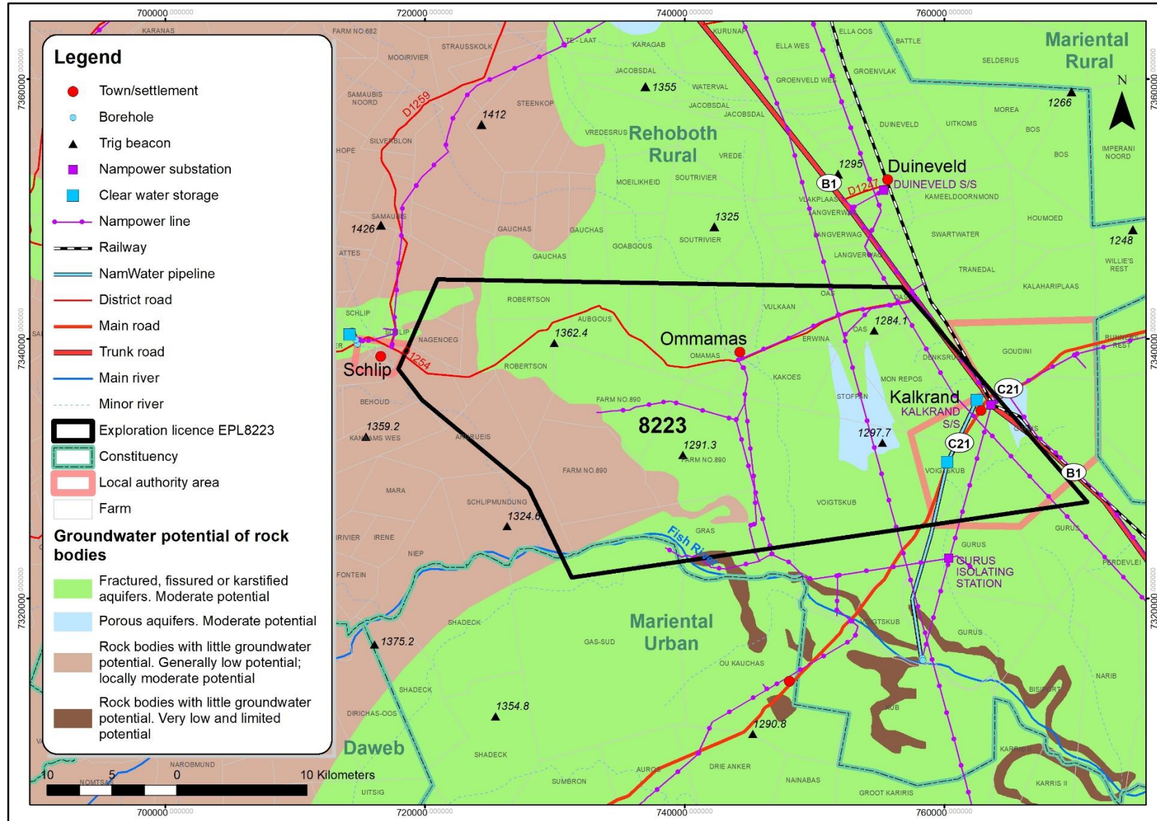
Figure 7: Simplified hydrogeological map of the EPL 8223 (RBS Map Prepared by Katharina Dierkes, 2021).
