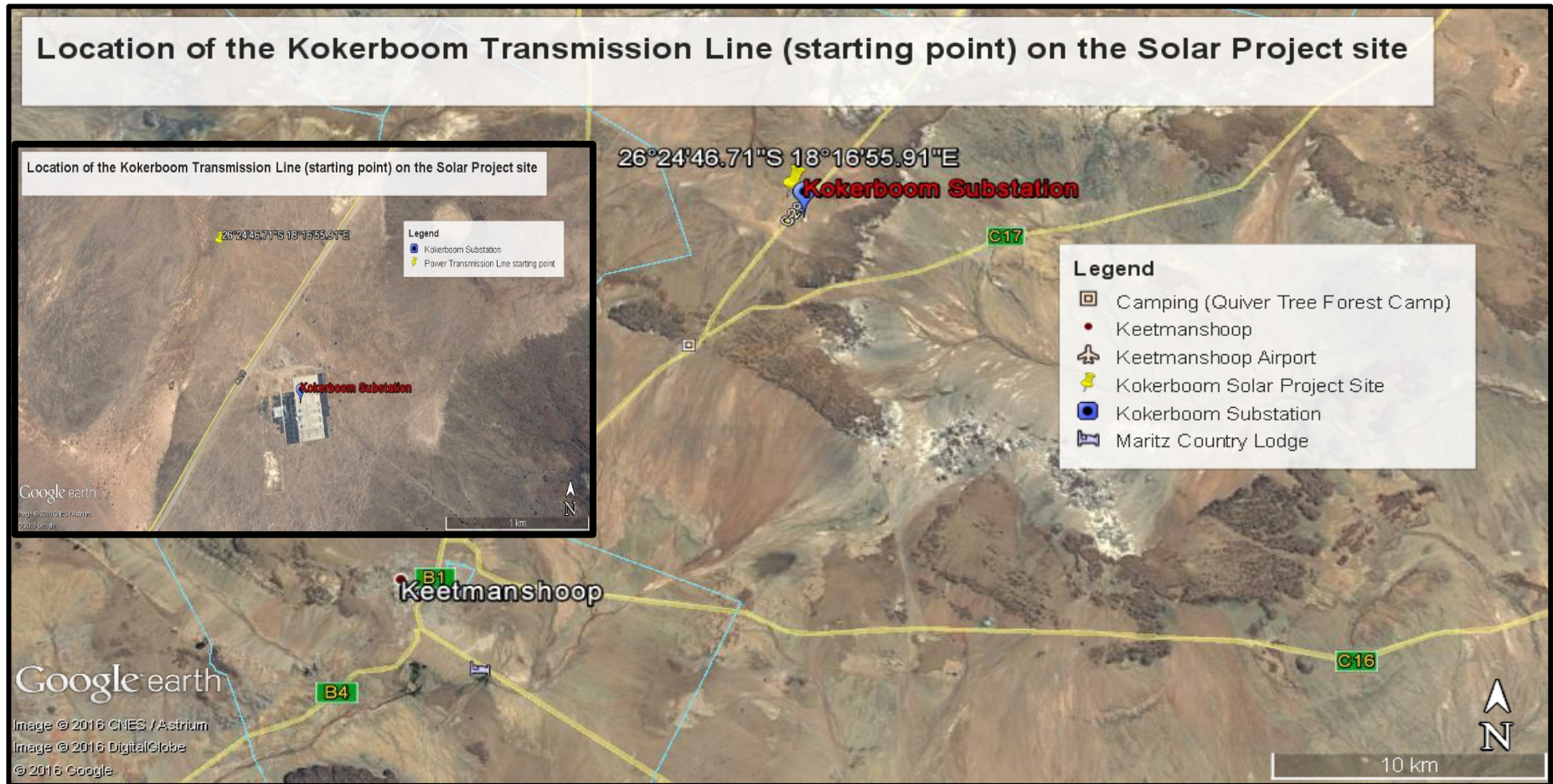
Location of the Kokerboom Transmission Line (starting point) on the Solar Project Site near Keetmanshoop, //Karas Region
