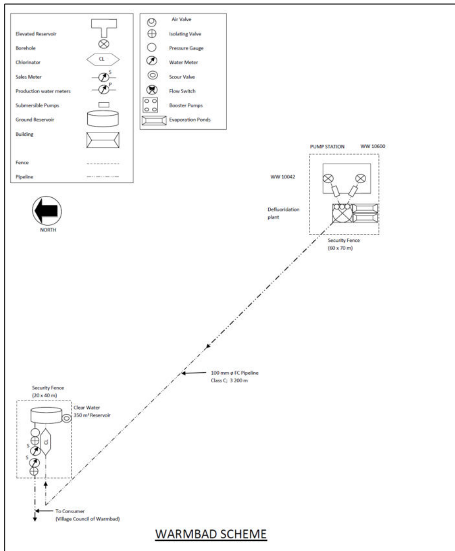
Figure 2: Warmbad Scheme Schematic Layout
