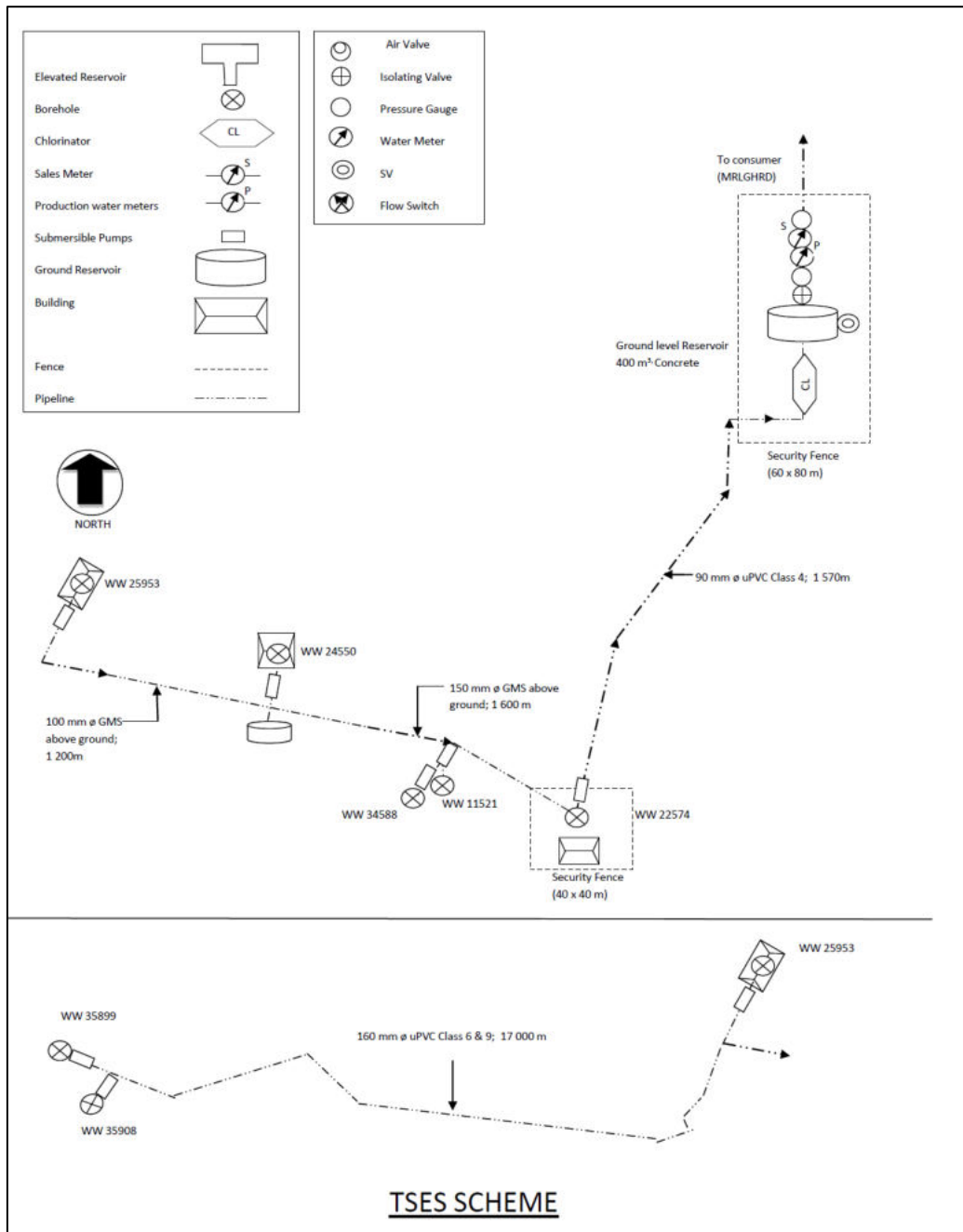
Figure 2: Tses Scheme Schematic Layout
