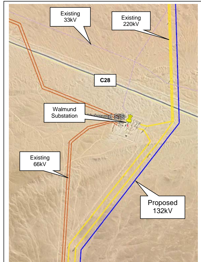
Figure 1.4 – OHTL Crossings around Walmund Substation
