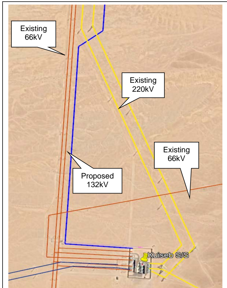
Figure 1.3 – OHTL Crossings around Kuiseb Substation
