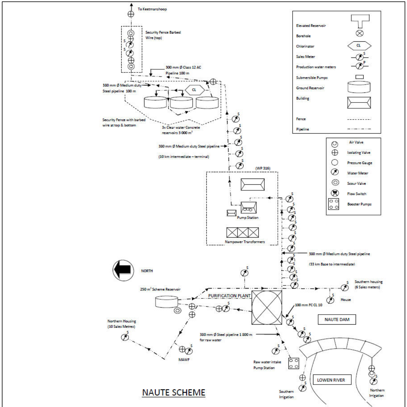
Figure 2: Naute-Keetmanshoop Scheme Schematic Layout
