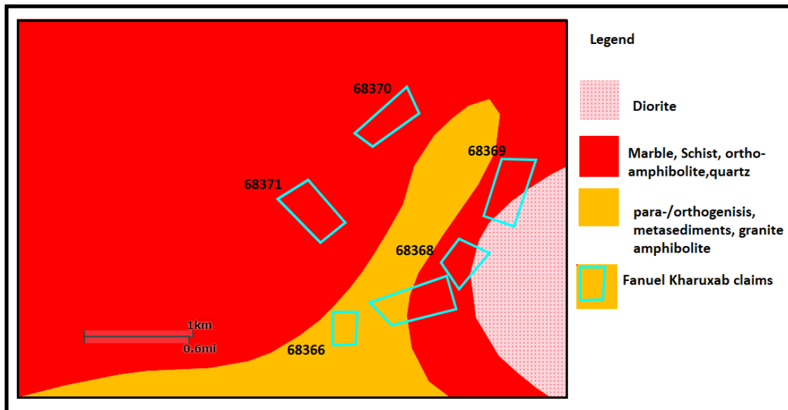
Figure 3: Geology of the proposed in Fanuel Kharuxab Mining Claims: 68366,68367,68368,68369,68370 and 68371site
