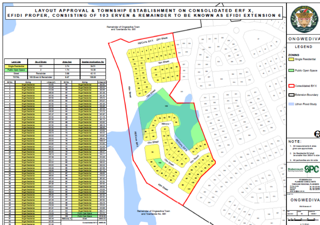
Figure 2: Layout of Proposed Efidi Extension 6
