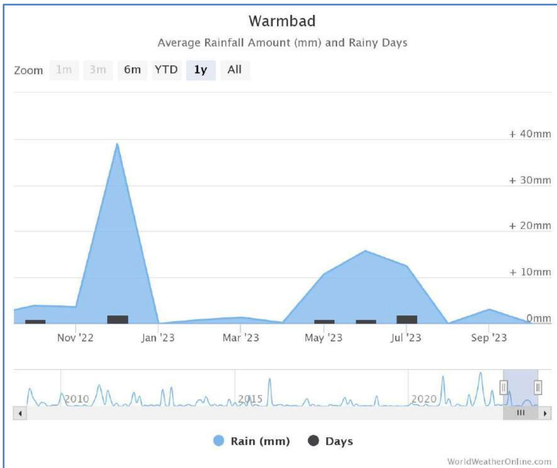
Figure 7 A graph showing rainfall patterns in Warmbad, from www.worldweatheronline.com
