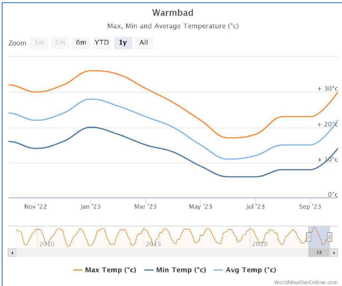
Figure 6 A graph showing the temperature patterns in Warmbad, from www.worldweatheronline.com Overall, winters are mild in temperature, with coldest month most often being June.
