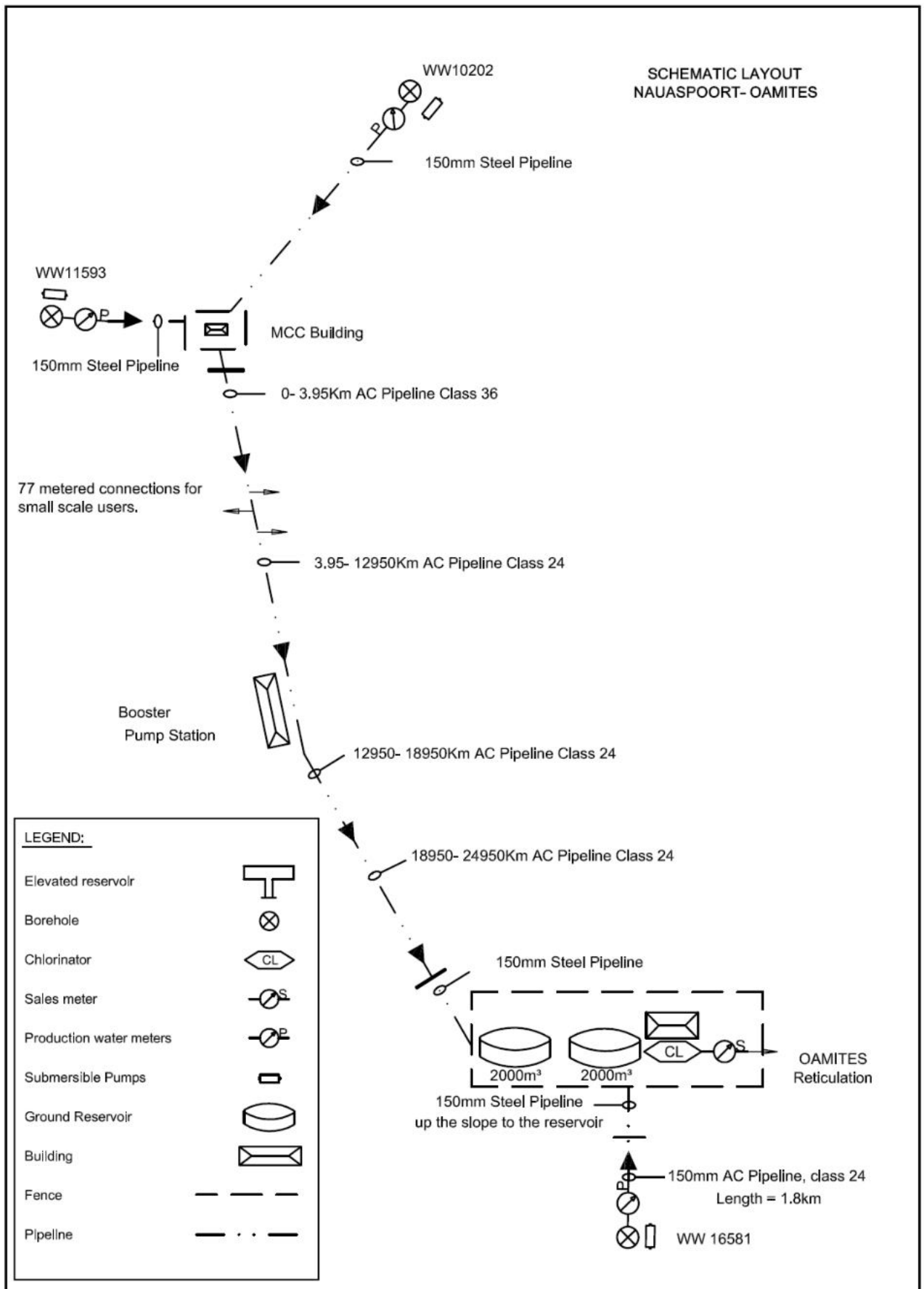
Figure 2: Nauaspoort-Oamites Scheme Schematic
