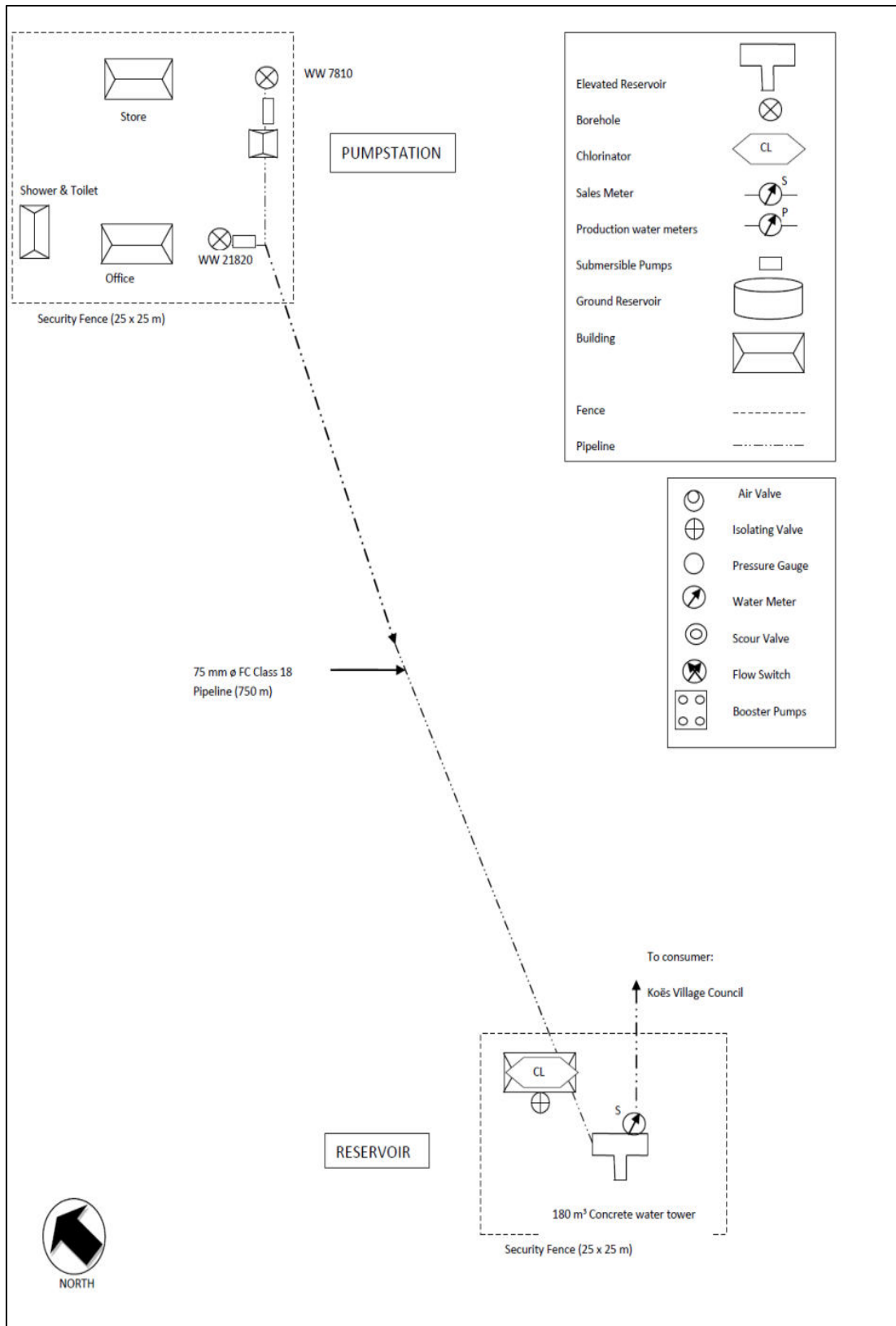
Figure 2: Kosis Scheme Schematic Layout
