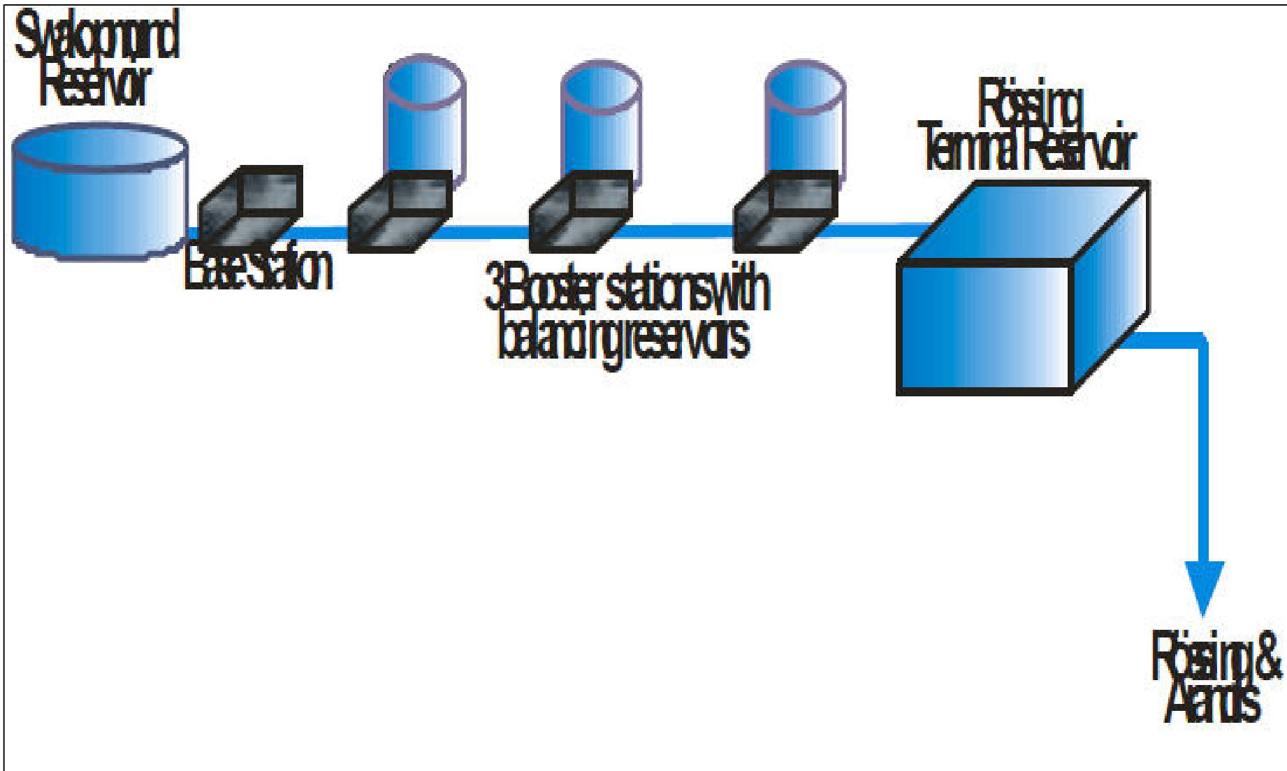
Figure 2: Swakopmund-Rössing Scheme Layout
