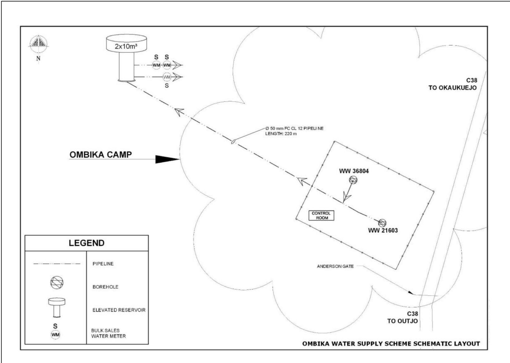
Figure 2: Ombika Scheme Layout
