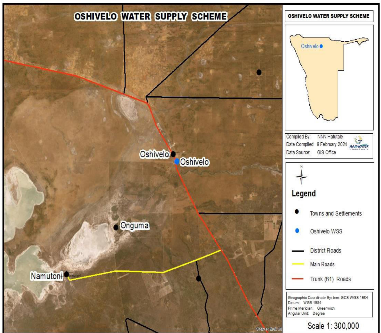
Figure 1: Oshivelo Location Map
