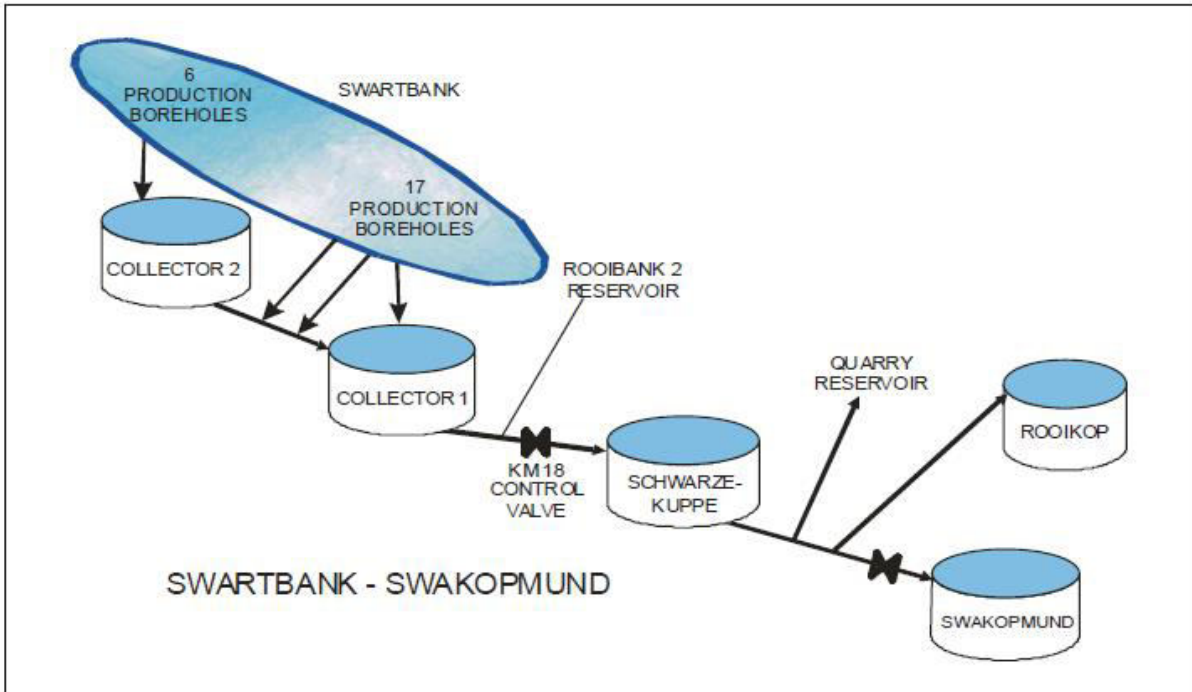
Figure 3: Schematic Layout of the Swartbank – Swakopmund Component
