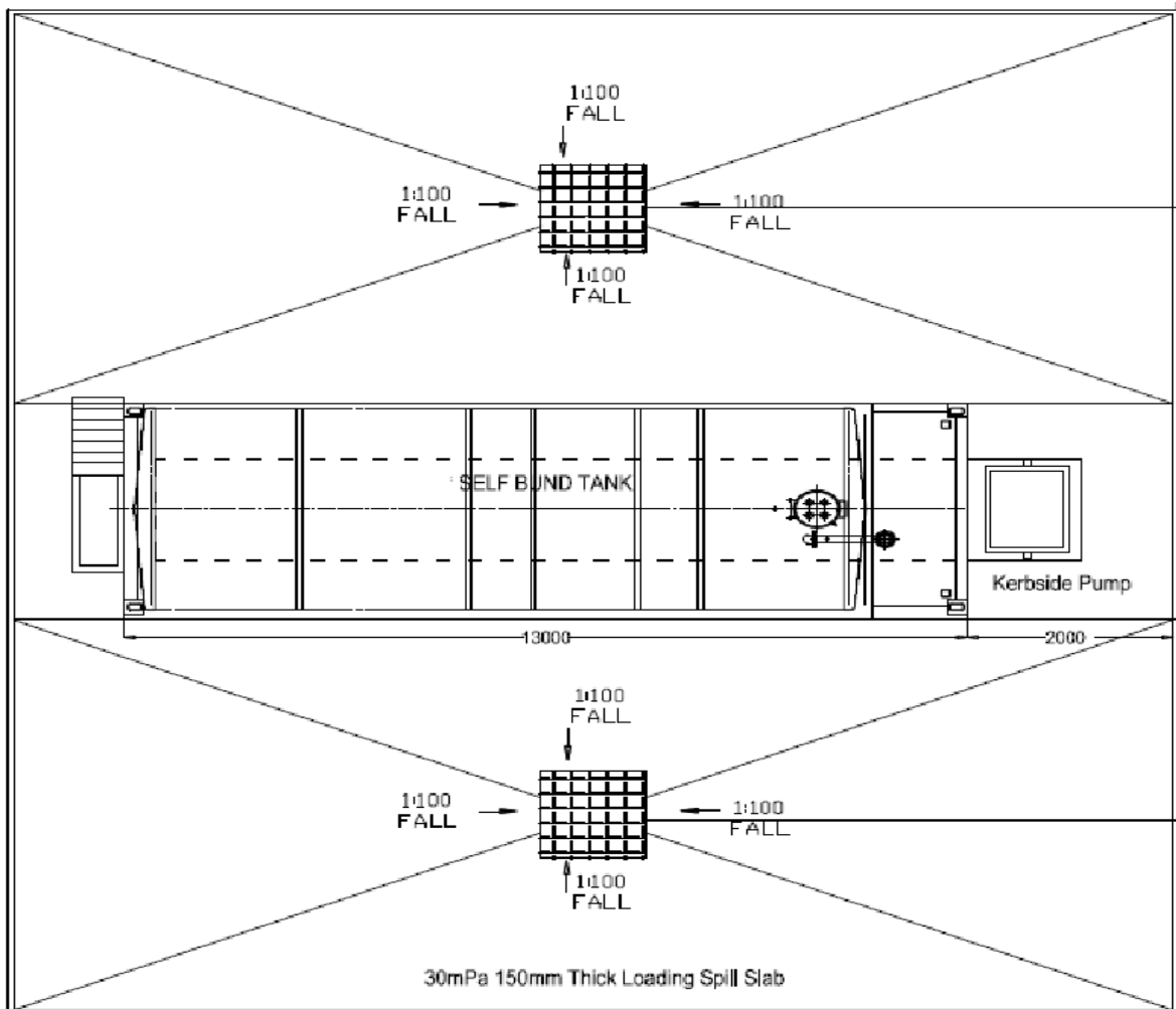
Figure 2. Proposed layout plan of the facility
