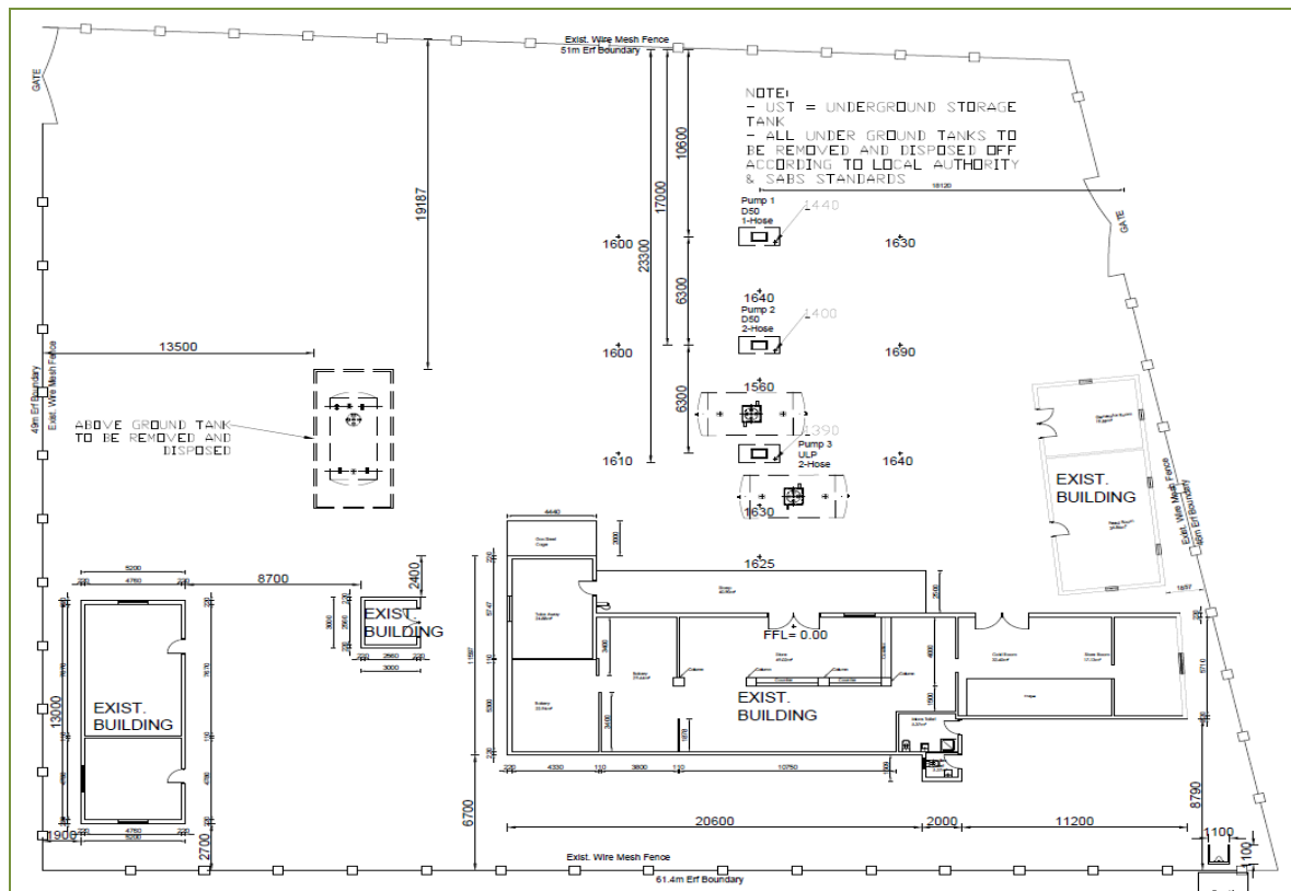
Figure 2. Current layout plan of the facility
