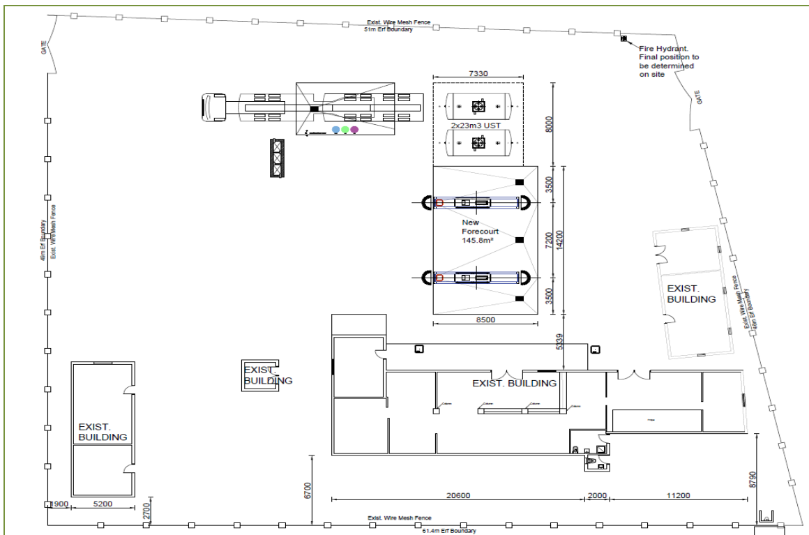
Figure 3. Proposed new layout plan of the facility
