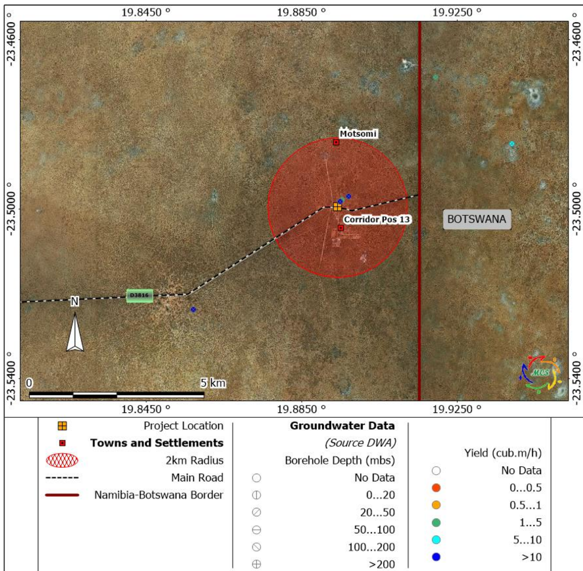
Figure 5. Hydrogeology of Area
