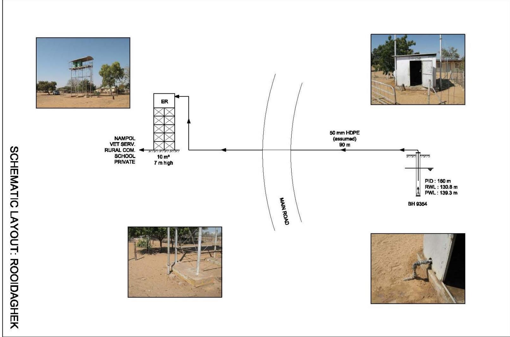
Figure 2: Rooidaghek Scheme Layout
