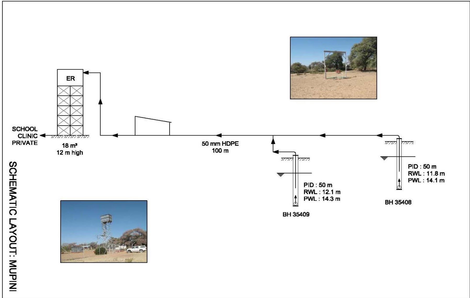
Figure 2: Mupini Scheme Layout
