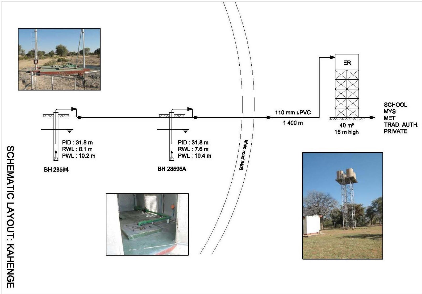
Figure 2: Kahenge Scheme Layout
