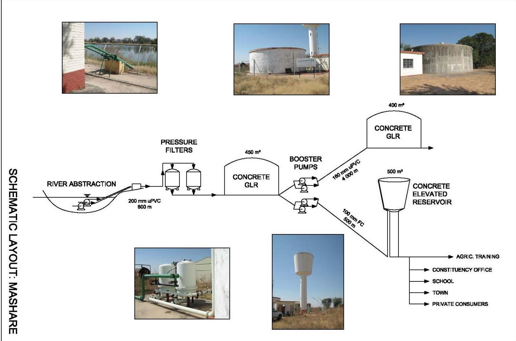
Figure 2: Mashere Scheme Layout
