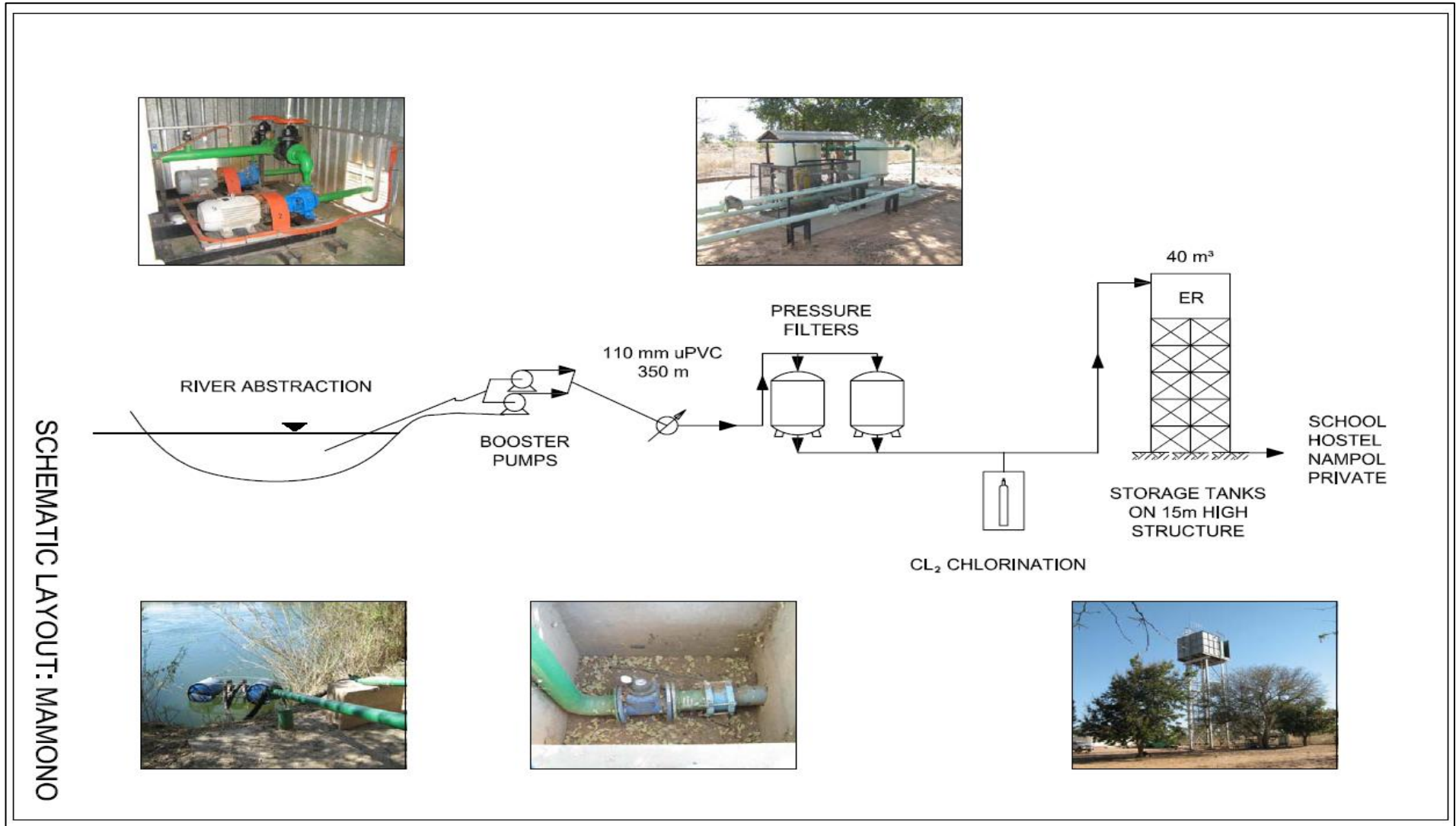
Figure 2: Mamano Scheme Layout
