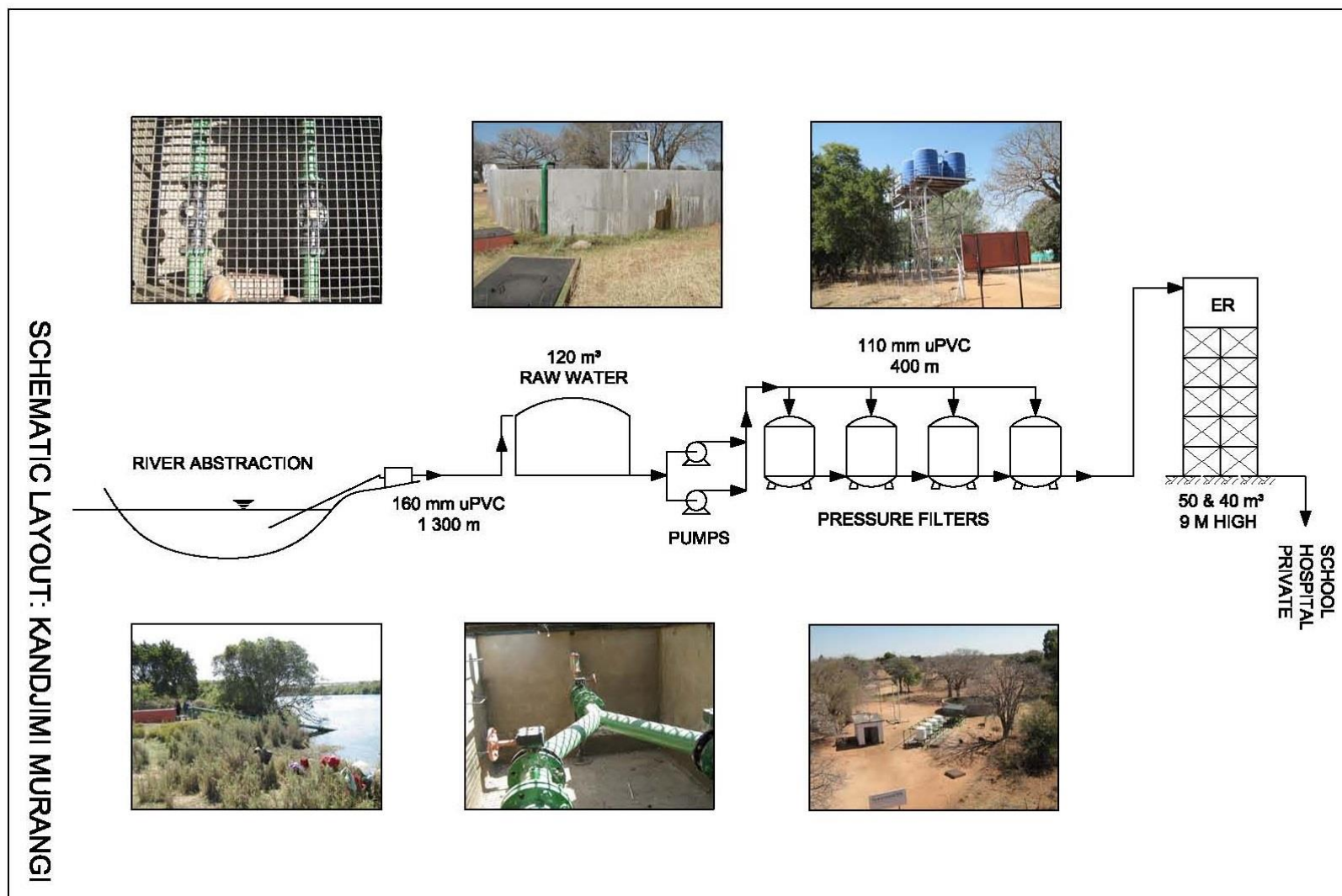
Figure 2: Kandjimi Murangi Scheme Layout
