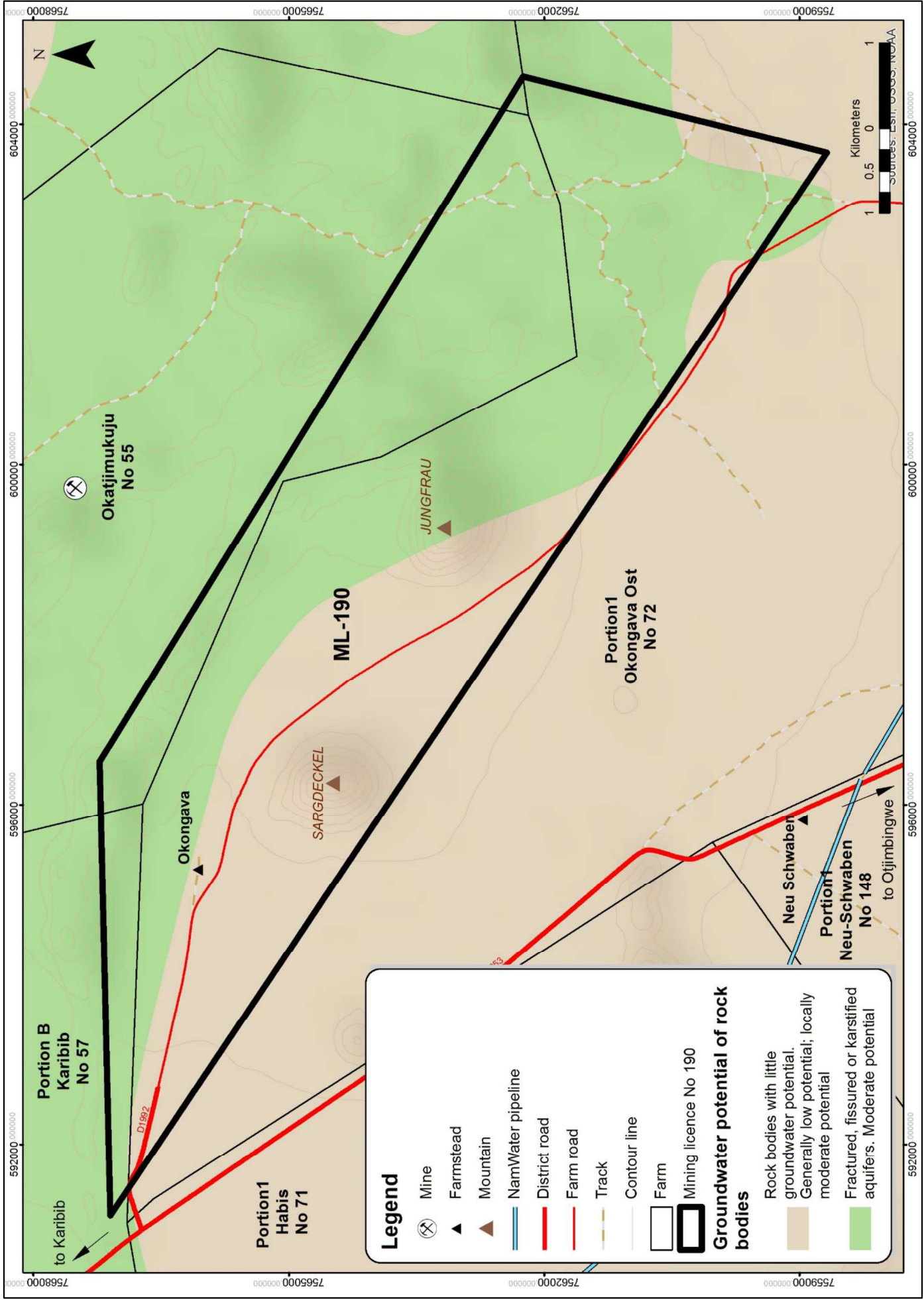
Figure 1.7: Simplified local hydrogeological map of the ML 190 (RBS Map Prepared by Katharina Dierkes, 2020).
