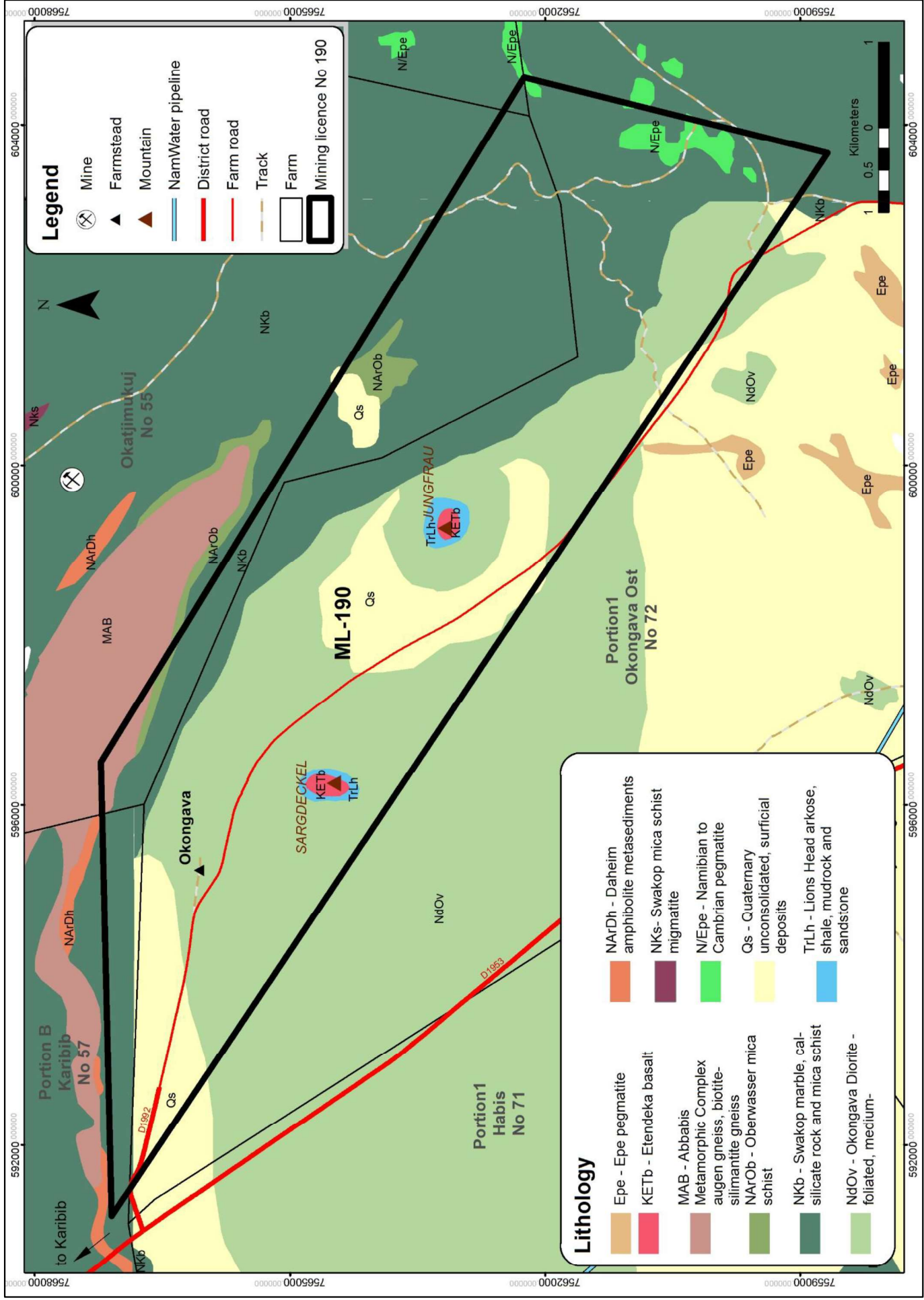
Figure 1.6: Simplified local geological map of the ML 190 (RBS Map Prepared by Katharina Dierkes, 2020).
