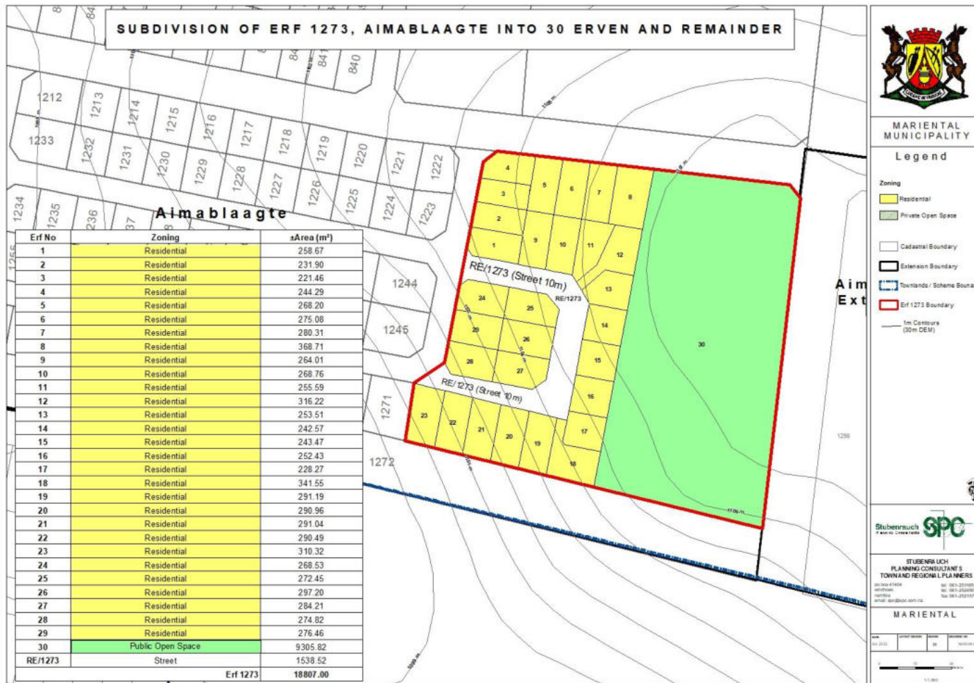
Figure 2-2: Layout Map for the proposed Subdivision of Erf 1273, Aimablaagte into 30 Erven and the Remainder
