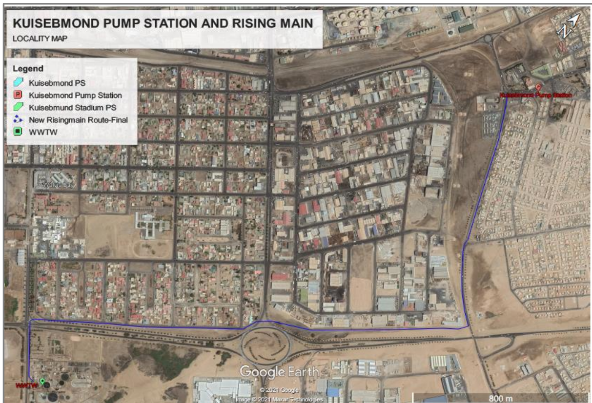
Figure 2. Kuisebmond sewage pump station and rising main route
