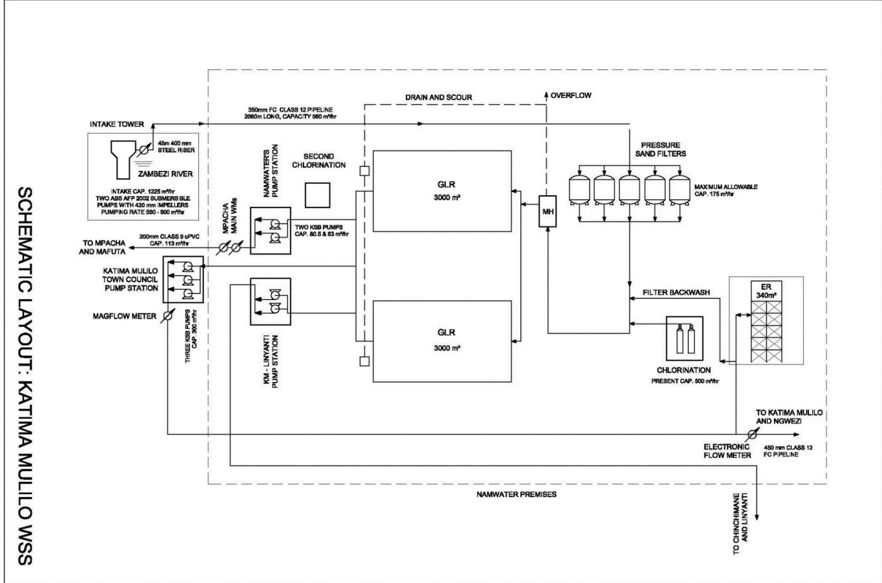
Figure 2: Katima Mulilo-Linyanti Scheme Layout
