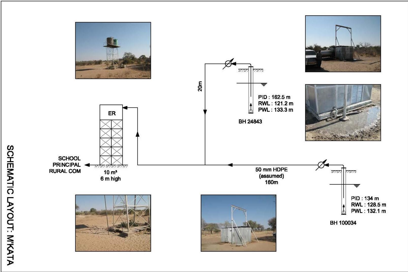
Figure 2: M'kata Scheme Layout
