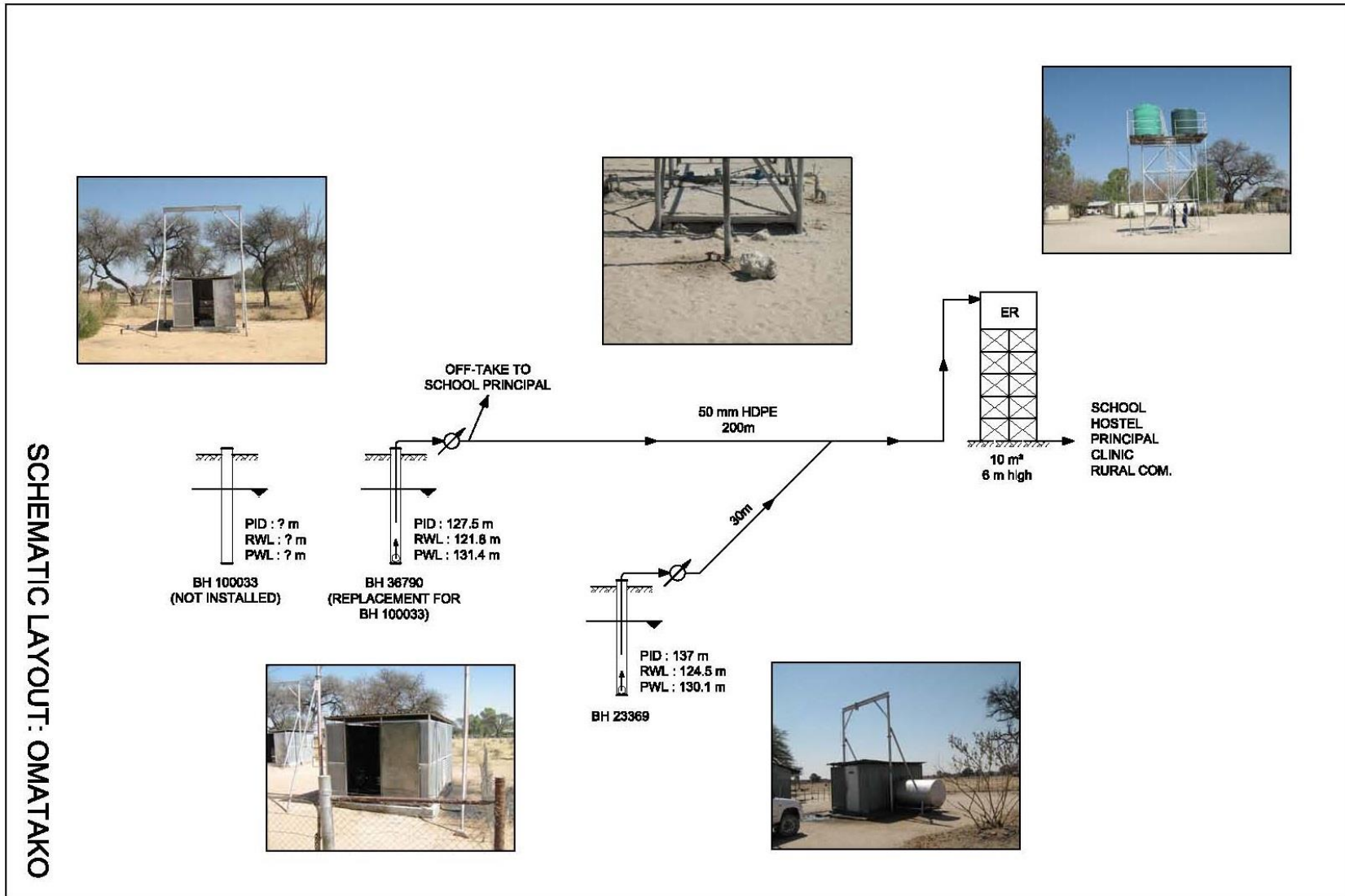
Figure 2: Omatako Scheme Layout
