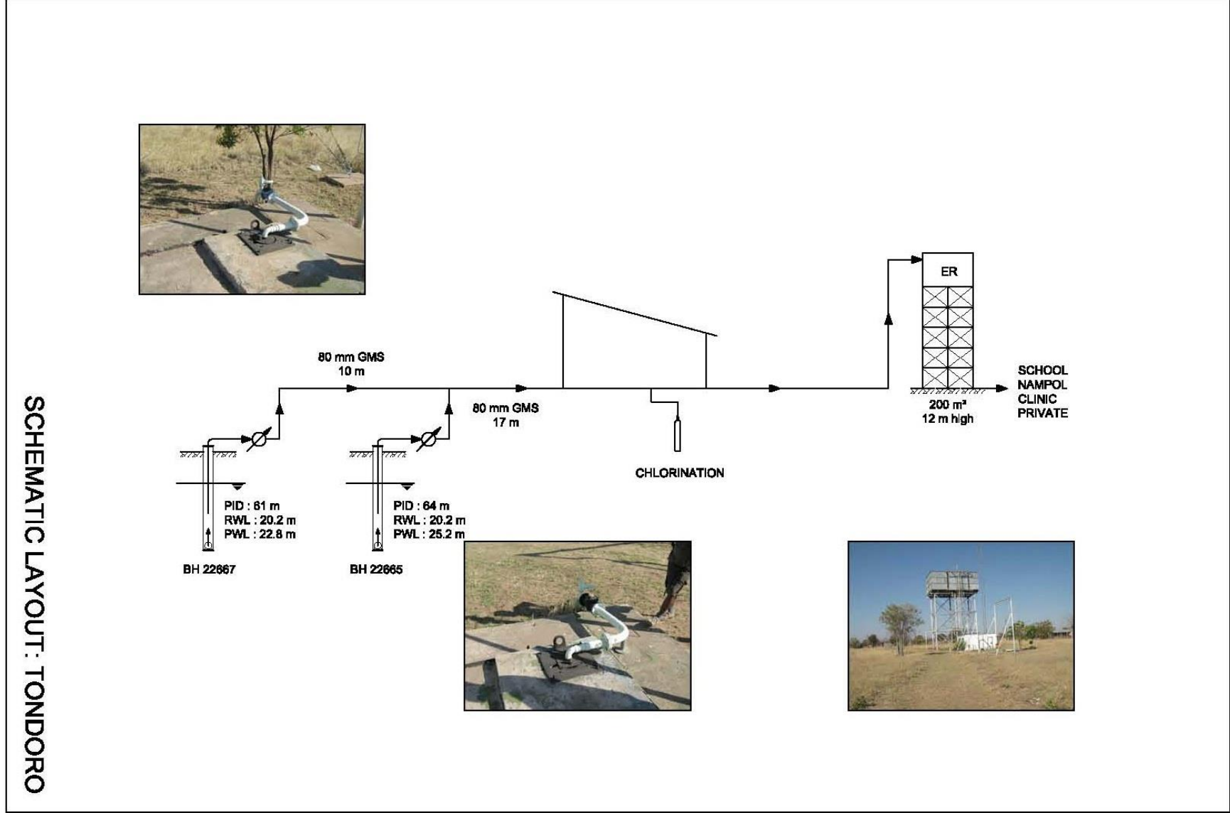
Figure 2: Tondoro Scheme Layout
