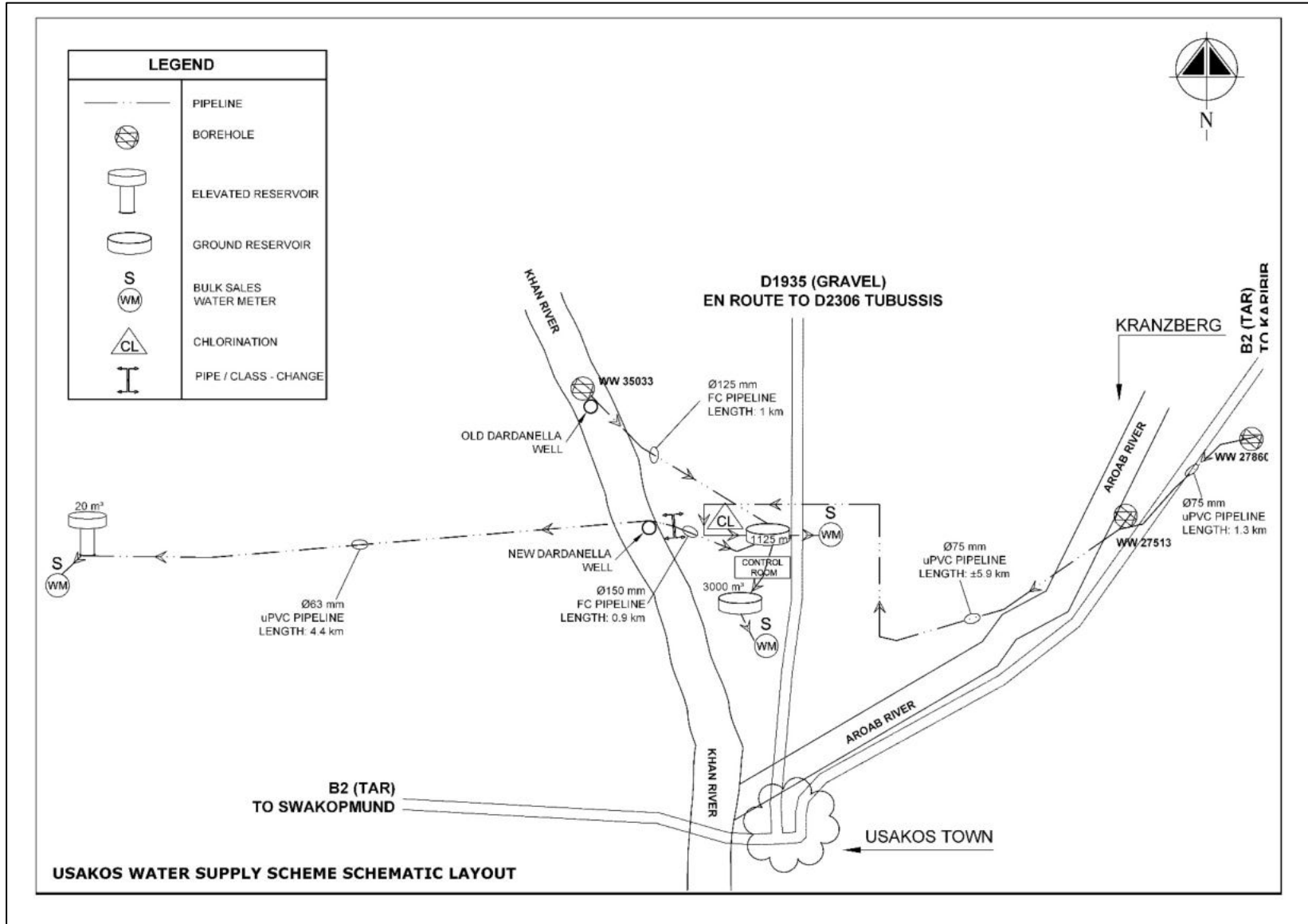
Figure 2: Usakos Scheme Layout
