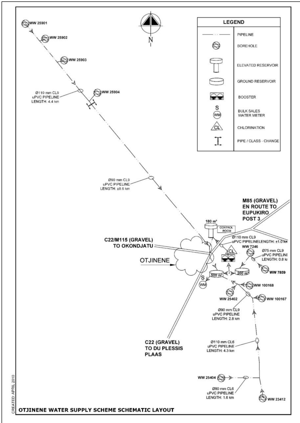
Figure 1: Otjovasandu Scheme Layout
