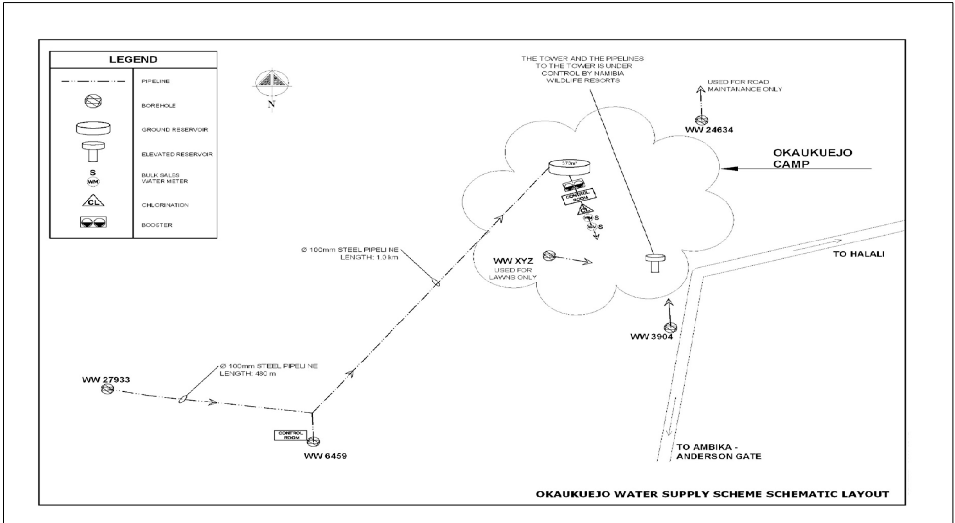
Figure 2: Okaukuejo Scheme Layout
