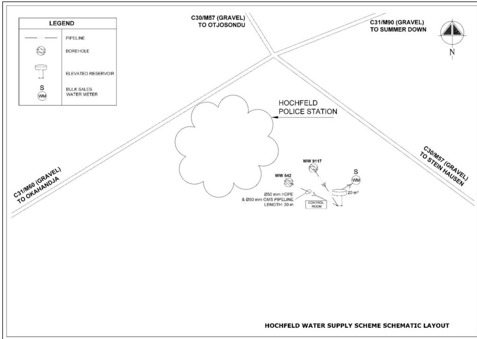
Figure 1: Hochfeld Scheme Layout
