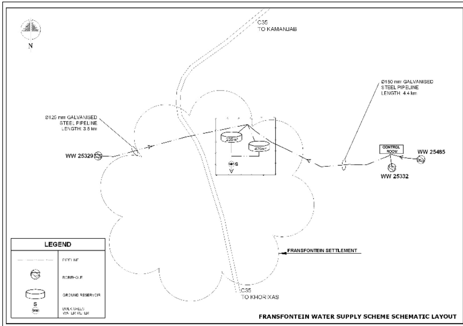
Figure 2: Fransfontein Scheme Layout
