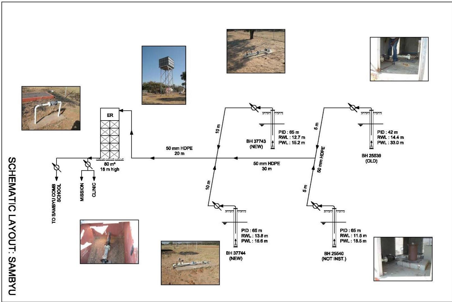
Figure 2: Sambyu Scheme Layout
