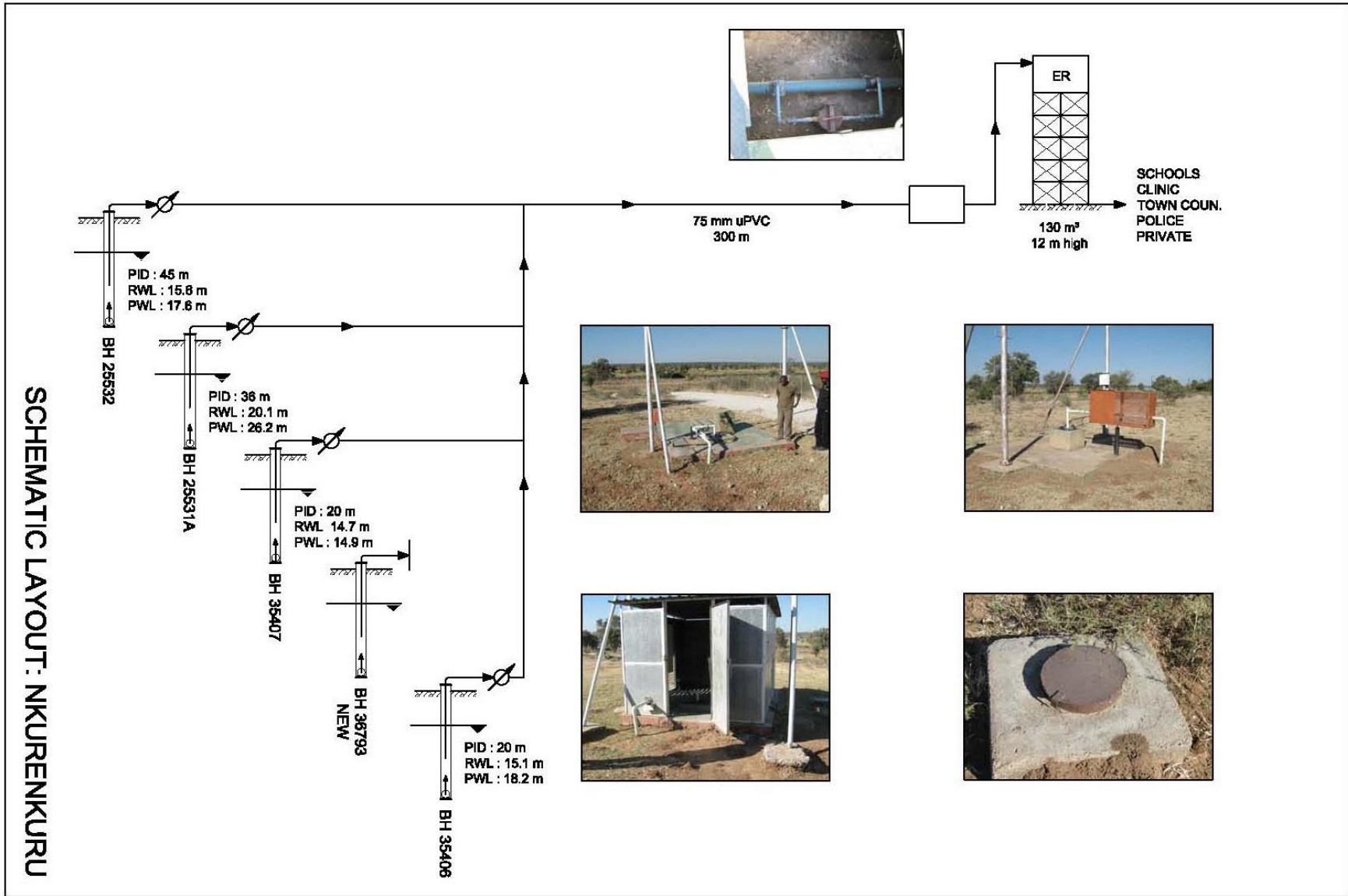
Figure 2: Nkurenkuru Scheme Layout
