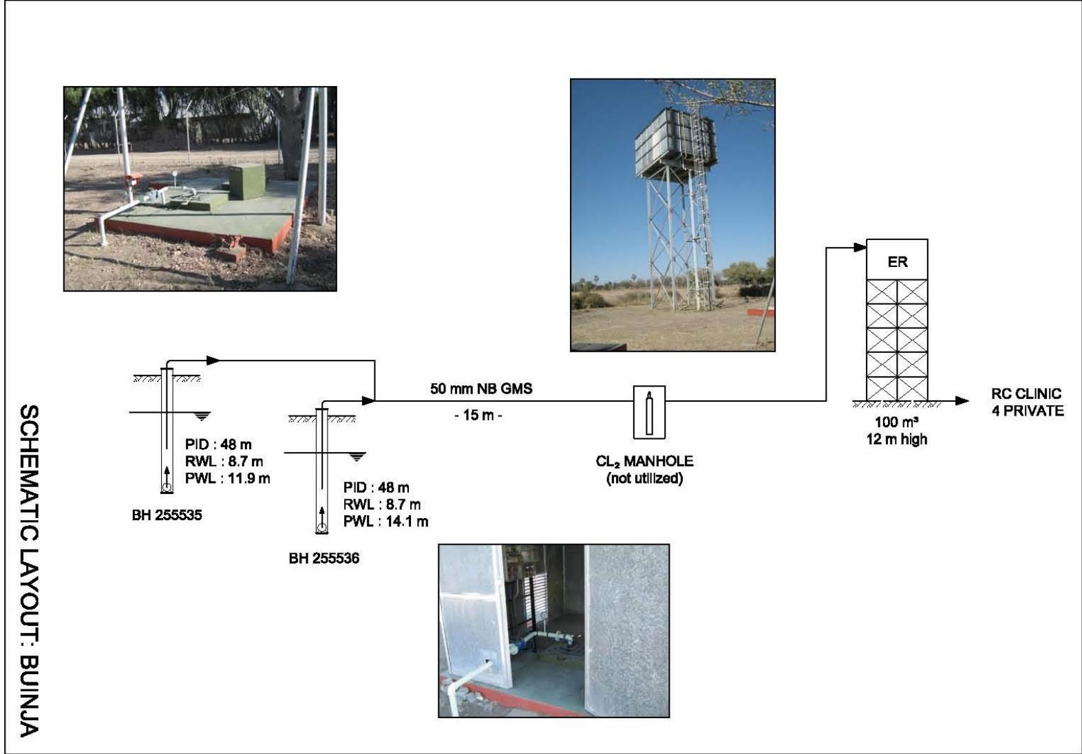
Figure 2: Buinja Scheme Layout
