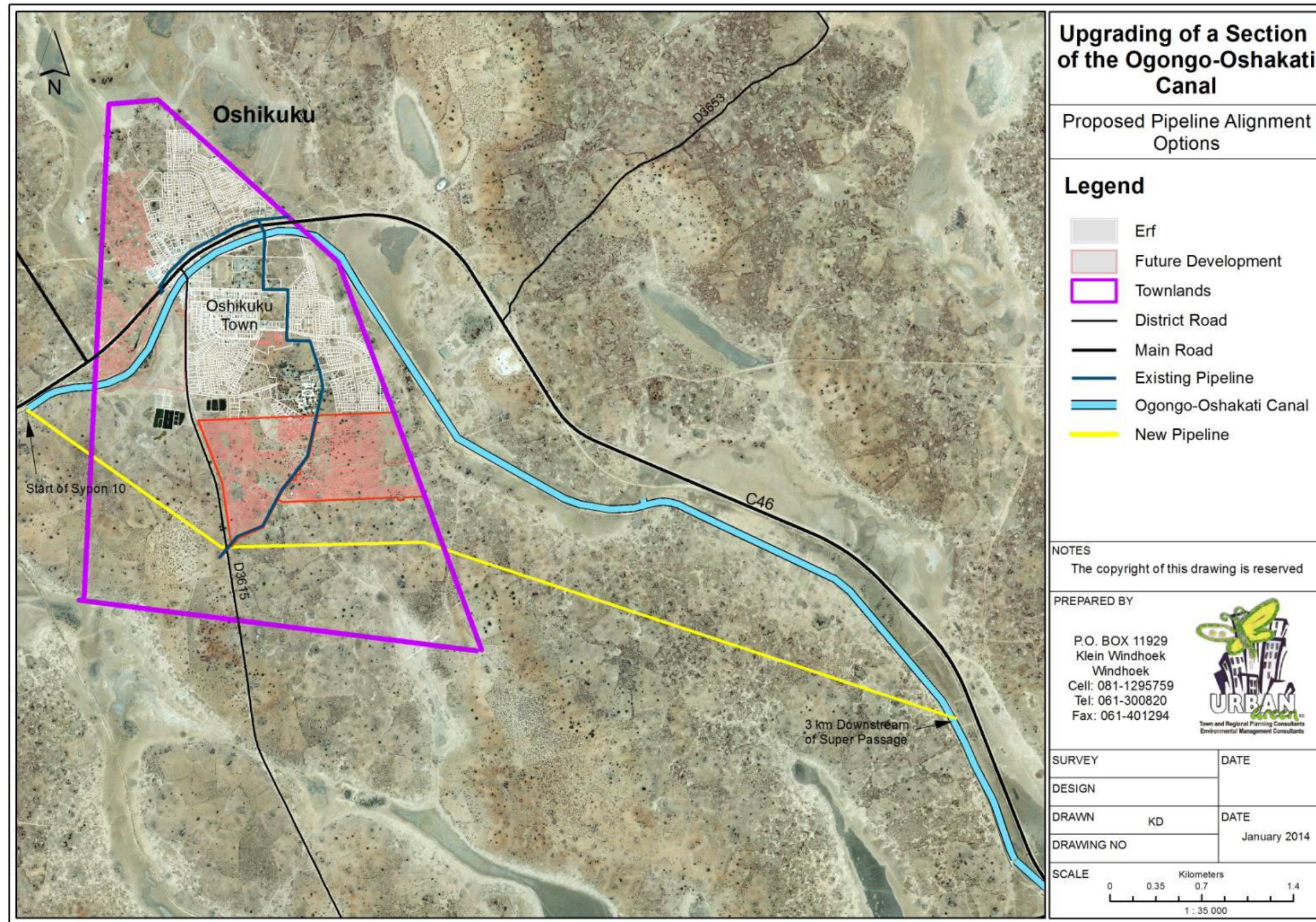
Figure 1: Locality of the problematic section of the Ogongo - Oshakati Canal (between siphon 10 and the Super passage) and the proposed direct new pipe line
