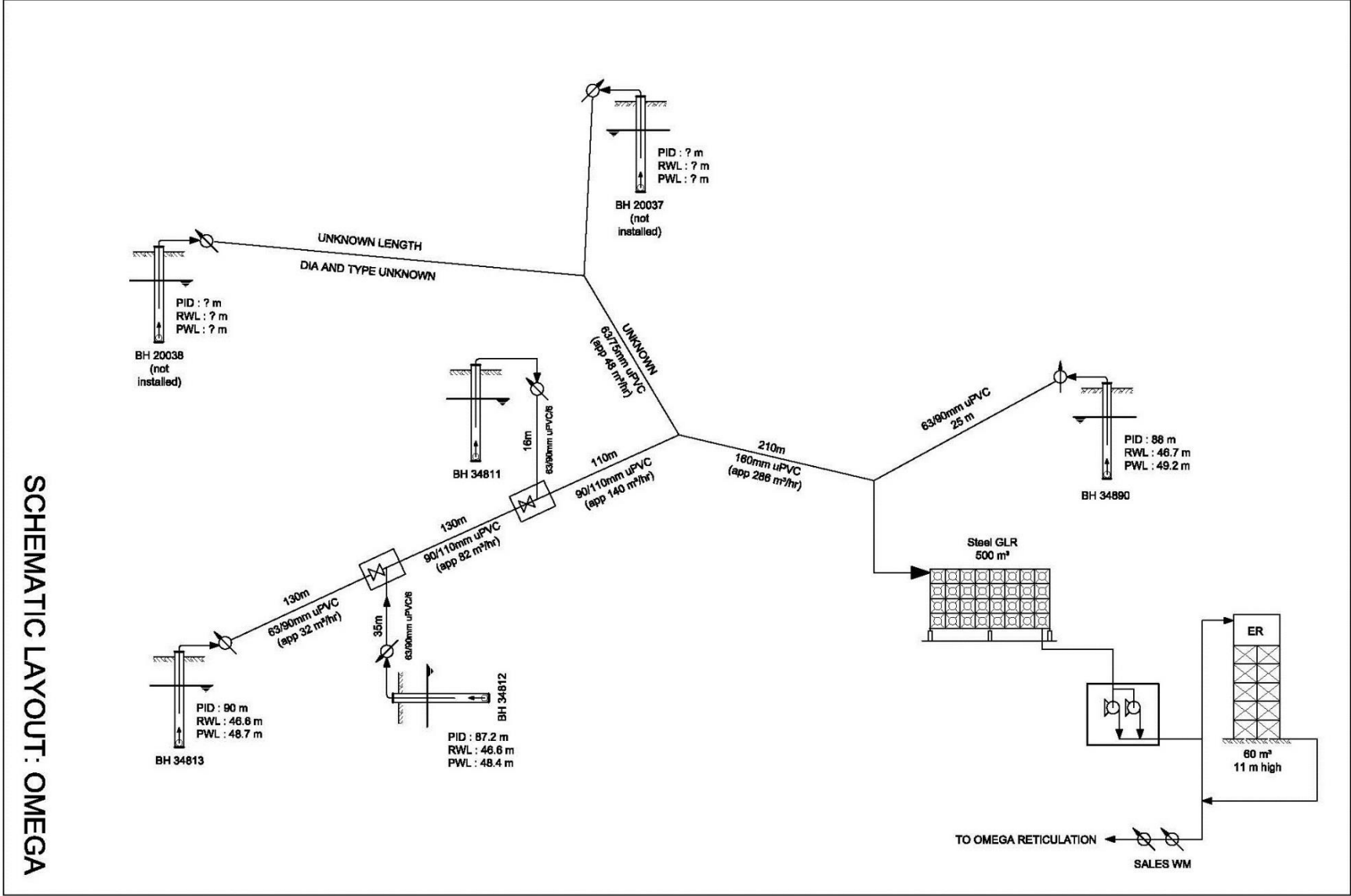
Figure 2: Omega Scheme Layout
