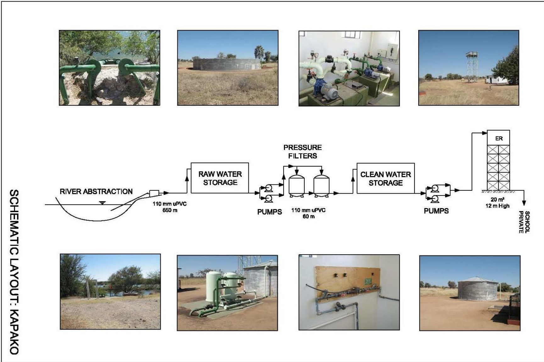
Figure 2: Kapako Scheme Layout
