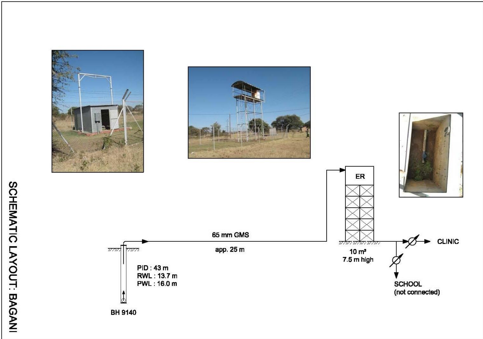
Figure 2: Bagani Scheme Layout
