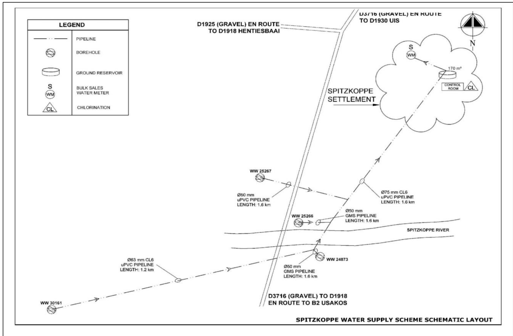
Figure 1: Spitzkoppe Scheme Layout
