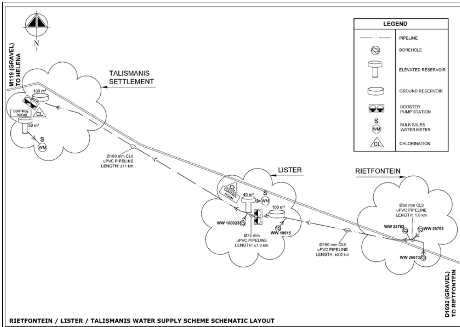
Figure 1: Rietfontein-Lister-Talismanis Scheme Layout
