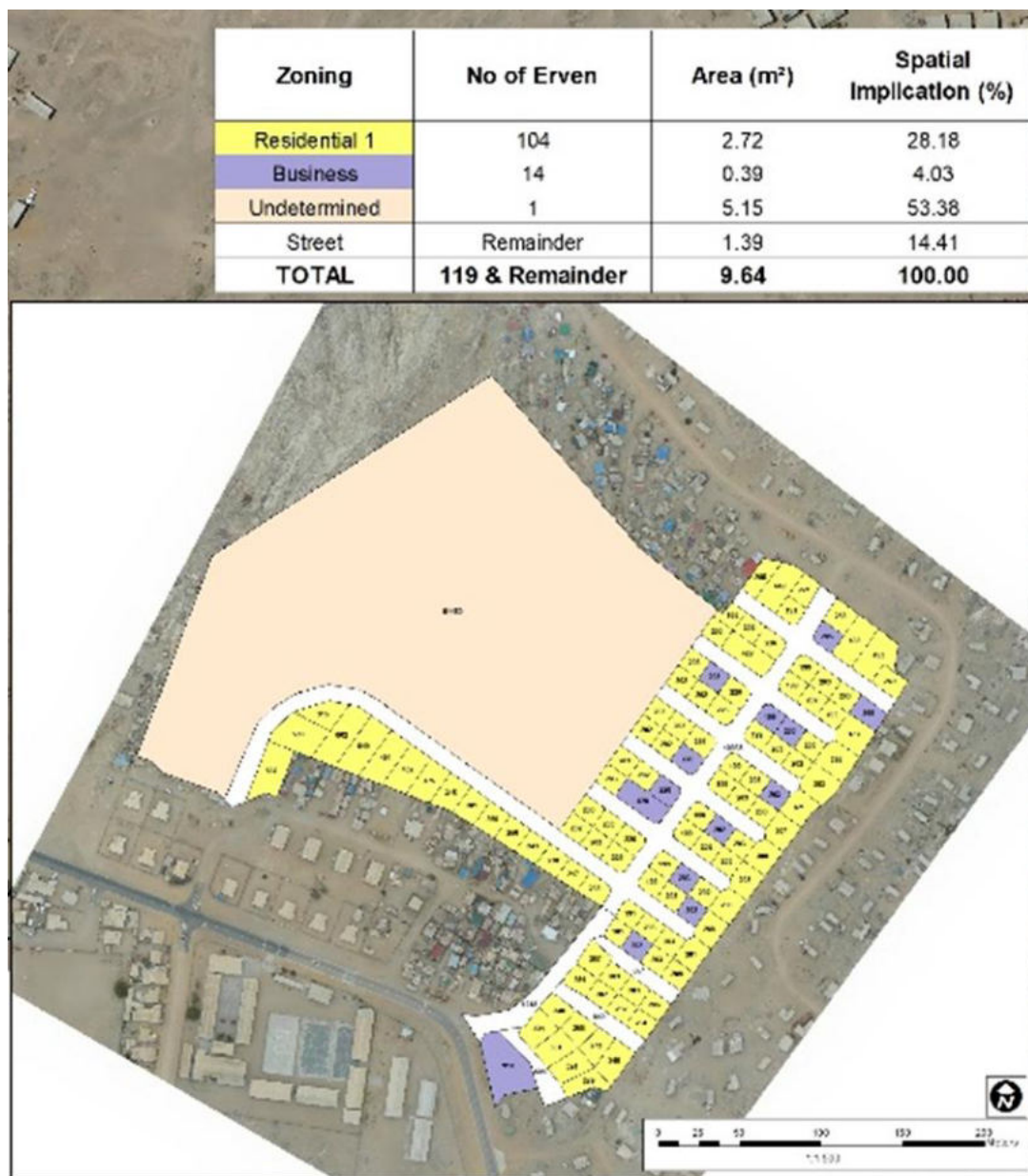
Figure 2: Draft layout of Benguela Extension 6
