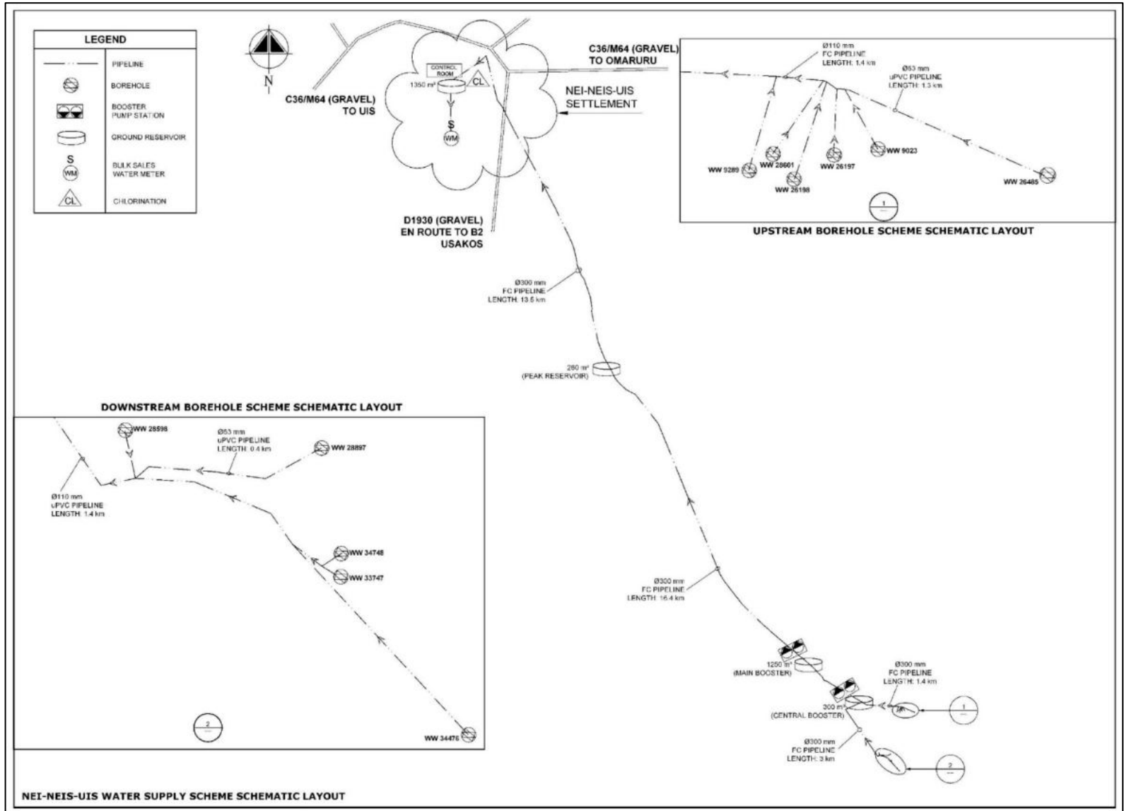
Figure 1: Nei-Neis Uis Scheme Layout
