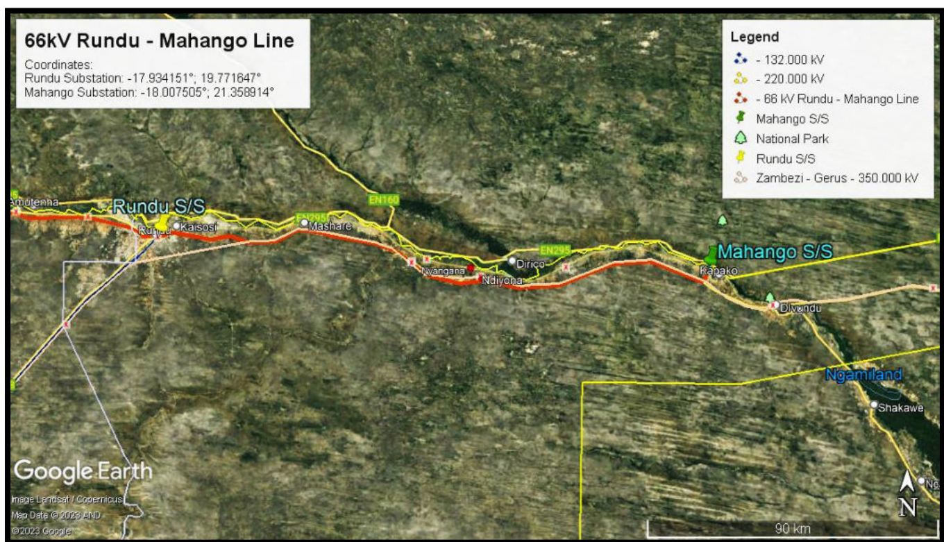
Figure 1: Locality map showing the 66 kV Rundu- Mahango transmission line
