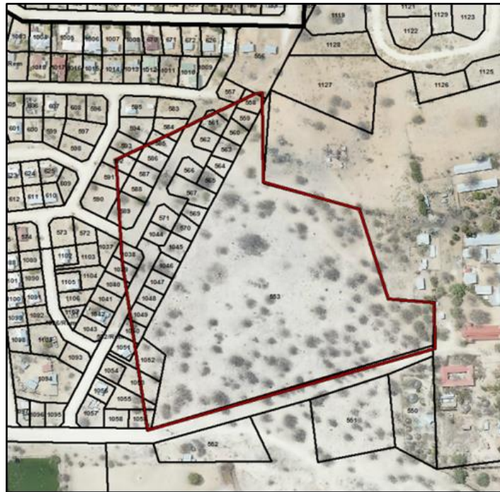
Figure 2: Cemetery encroachments on Oshikuku Extension 1
